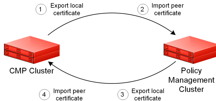
Figure 3-9 Exchanging Certificates
