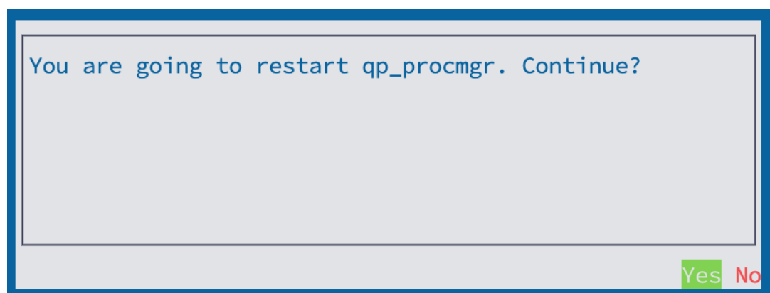
Figure 2-1 Restart qp_procmgr
