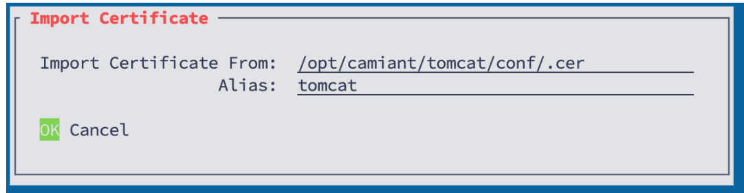
Figure 3-10 Import Certificate
