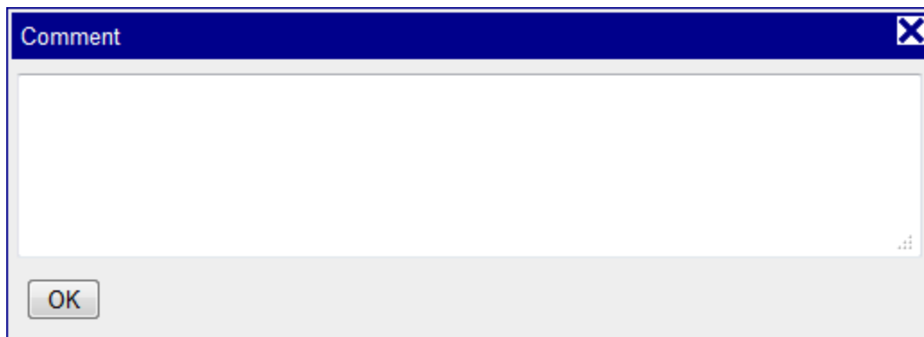
Figure 3 : Comment Dialog
