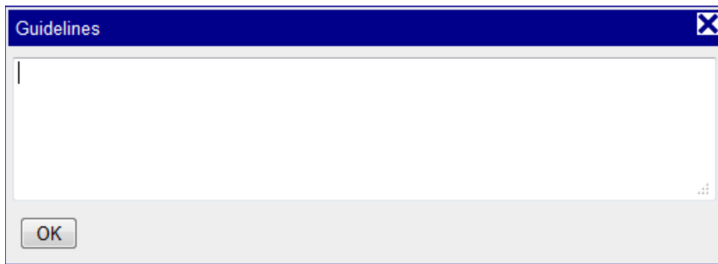
Figure 4 : Guidelines Dialog
