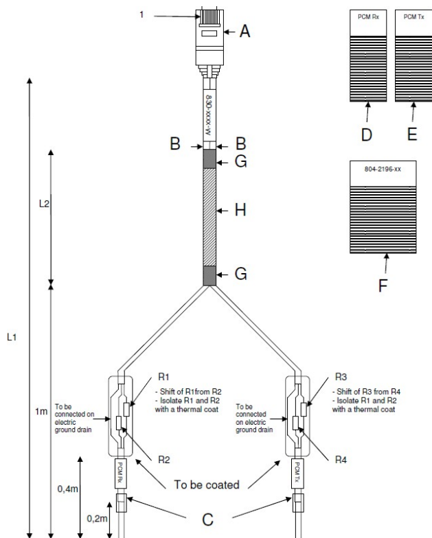
Figure 20- Cable for Falco: sample configuration for unprotected links
