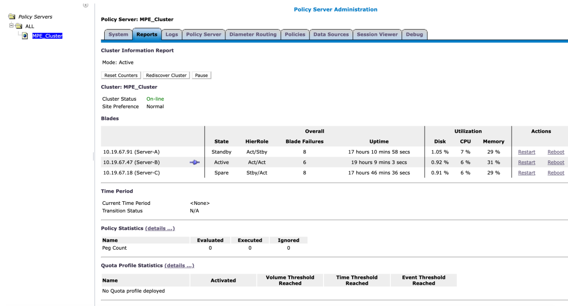
Figure 3-1 Statistics Displayed Over a Secure Connection
