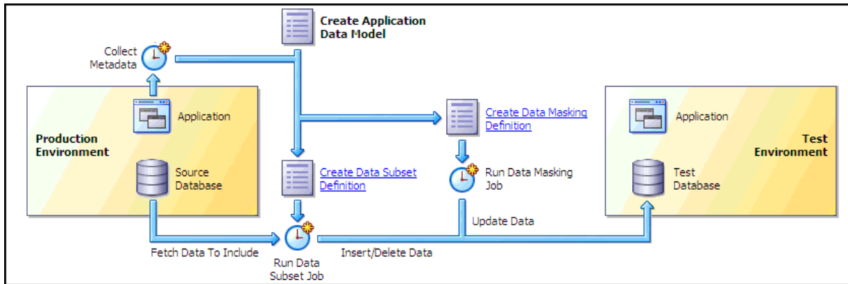
Figure 3-2 Test Data Management Architecture
