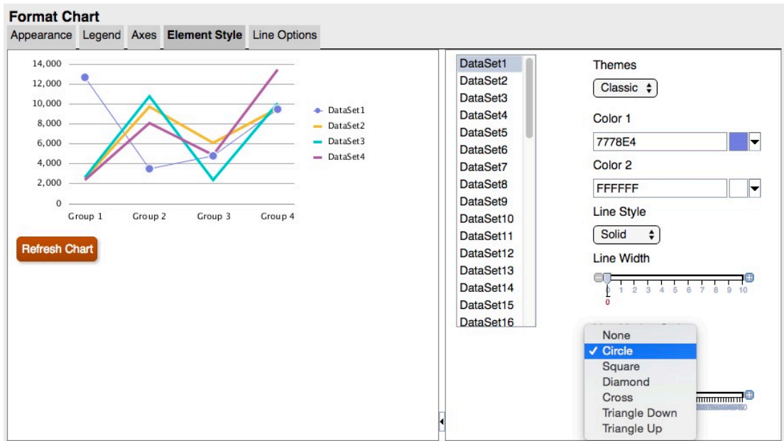
Figure 5-45 Line Marker Styles in the Updated Charting Engine
