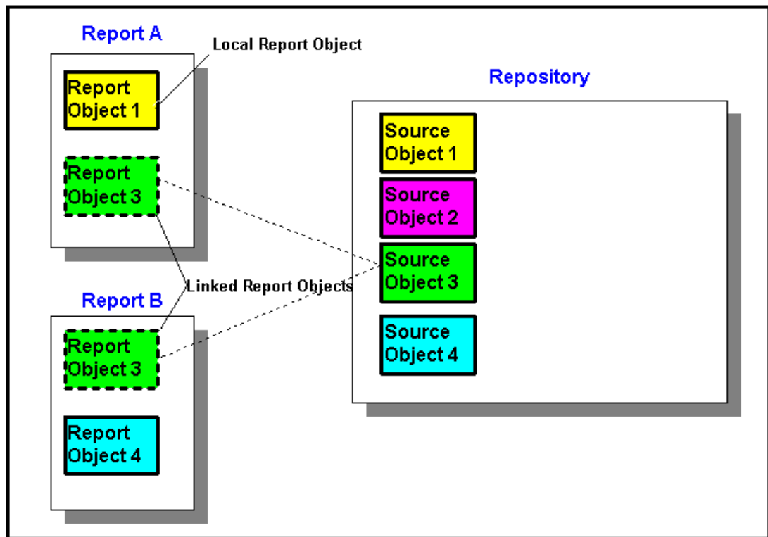
Figure 1-1 Linked and Local Report Objects
