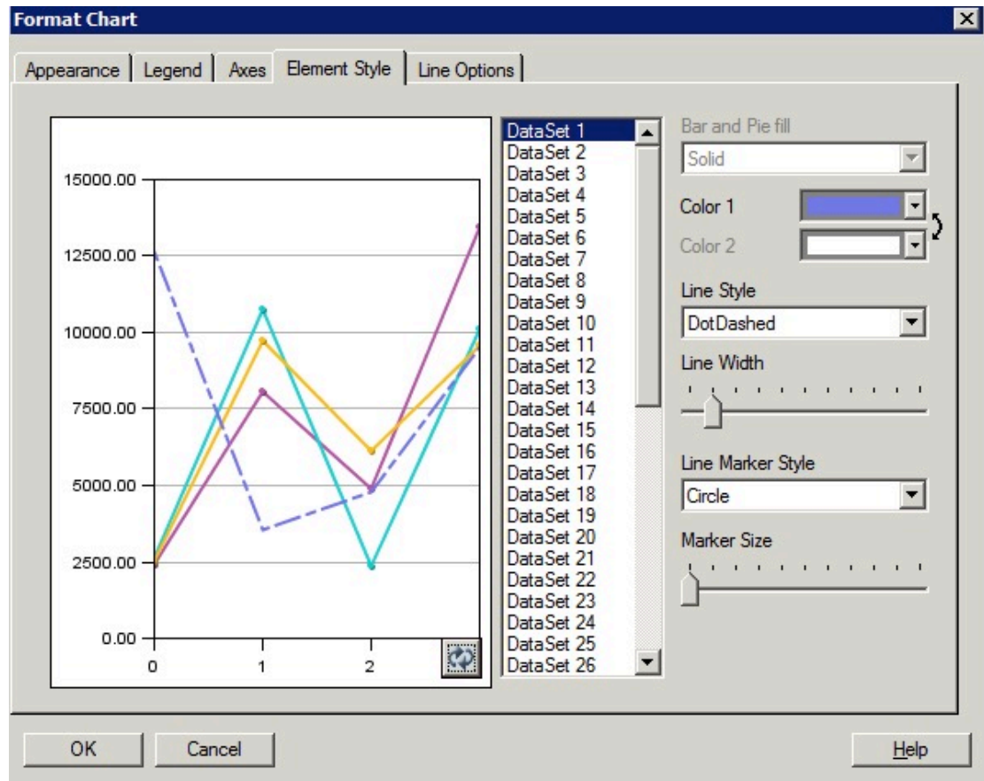
Figure 5-42 Element Style Tab in the Original Charting Engine Showing "DotDashed" as a Line Style
