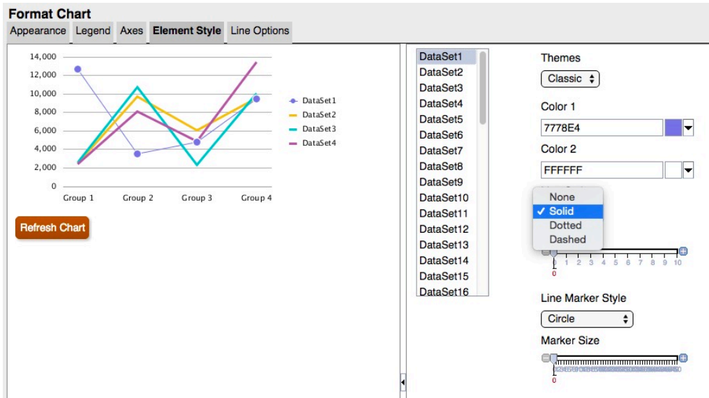
Figure 5-43 Element Style Tab in the Updated Charting Engine Showing That There is No "DotDashed" Line Style
