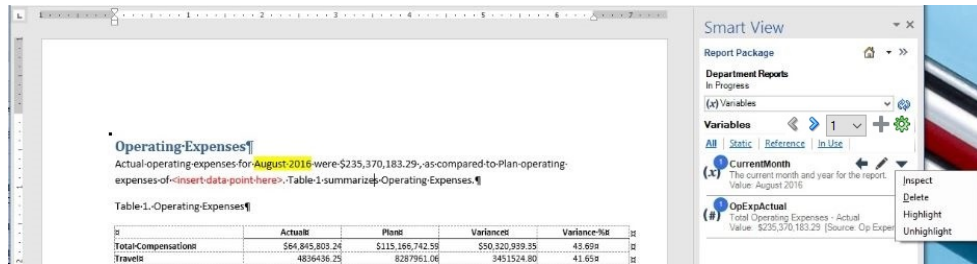
Figure 19-40 Doclet with Highlighting Enabled for a Selected Variable
