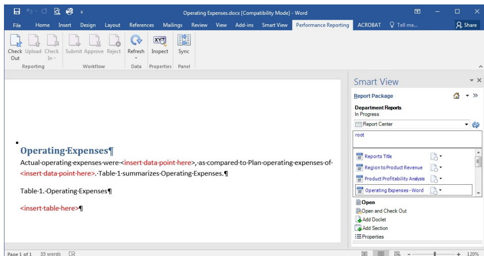
Figure 19-56 Doclet Opened from Smart View Panel, Ready to be Checked Out
