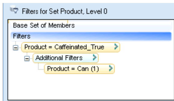
Figure 12-2 Intersection of Sets
