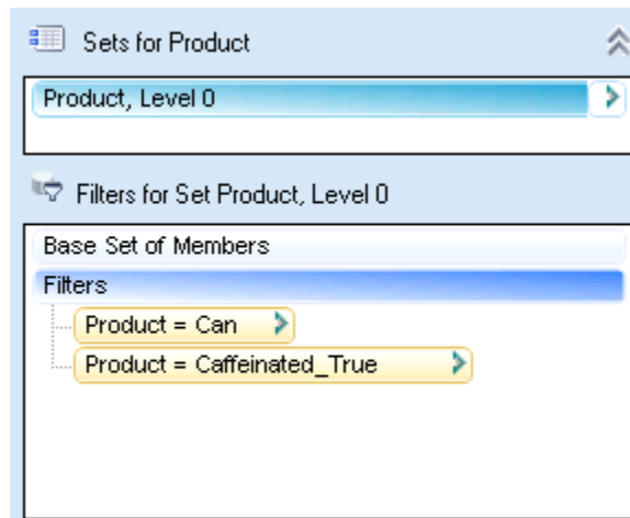
Figure 12-1 Union of Sets
