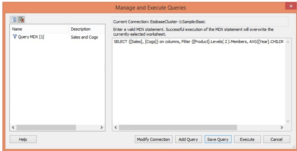
Figure 20-3 Newly-Saved MDX Query Listed in the Manage and Execute Queries Dialog Box
