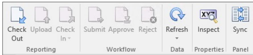
Figure 22-14 Narrative Reporting Ribbon for Doclet in Author Phase in Initial Unchecked-Out State
