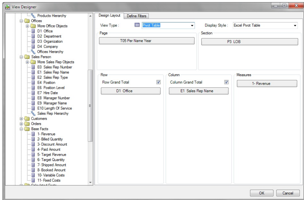
Figure 28-19 View Designer, Design Layout Tab for Pivot Table Layout
