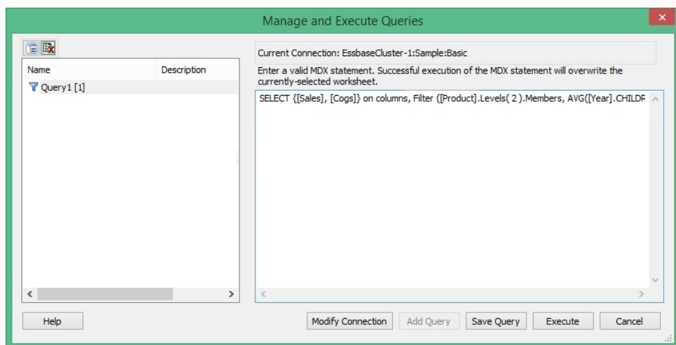
Figure 20-4 Manage and Execute Queries Dialog Box
