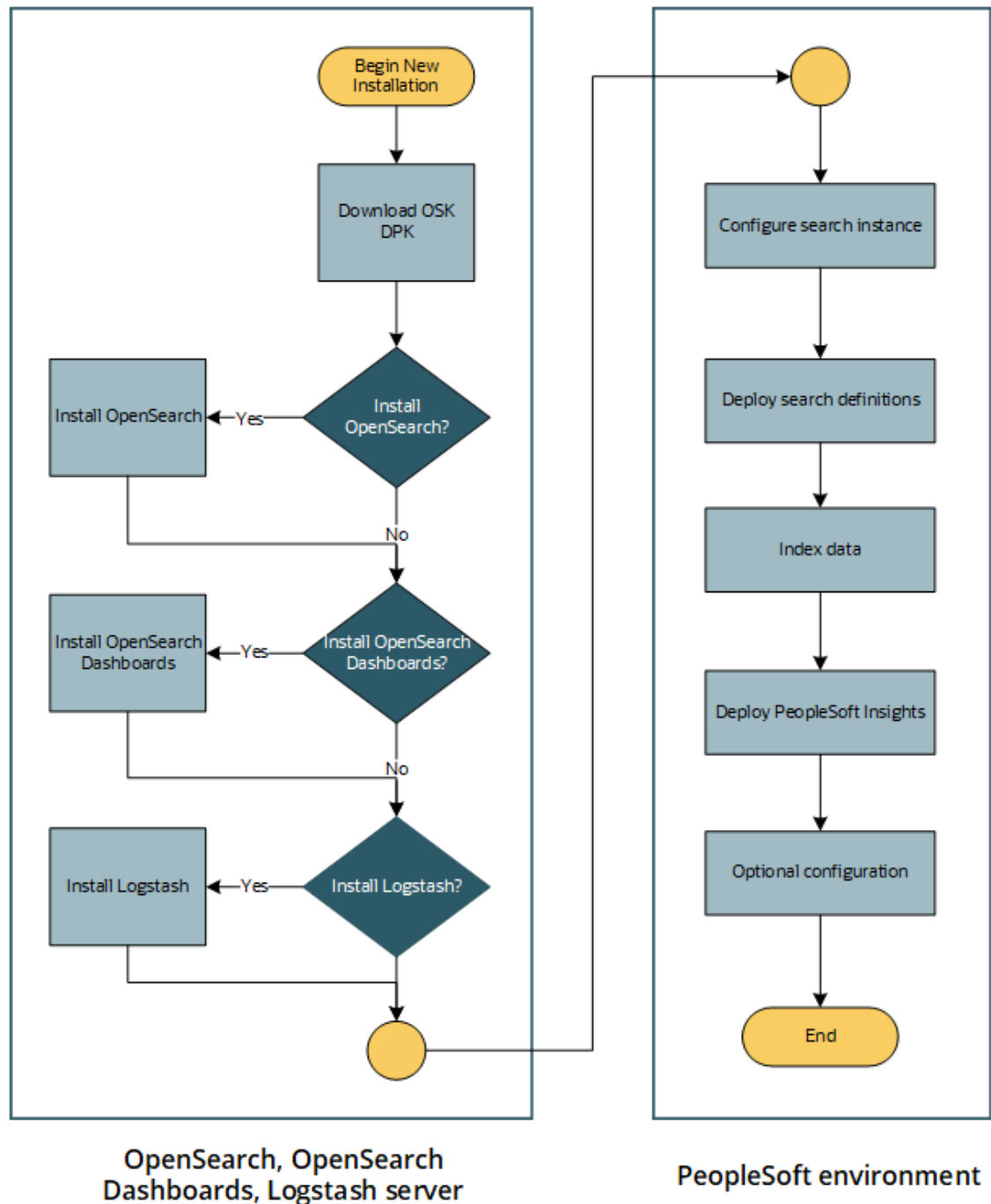
Figure 1-1 Deployment of OpenSearch, OpenSearch Dashboards, and Logstash
