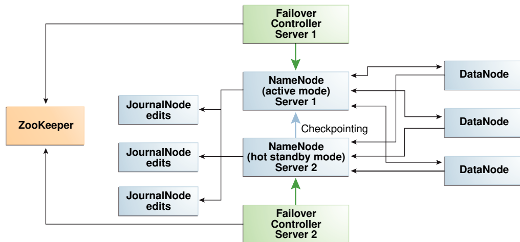
Figure 3-7 Automatic Failover of the NameNode on Oracle Big Data Appliance
