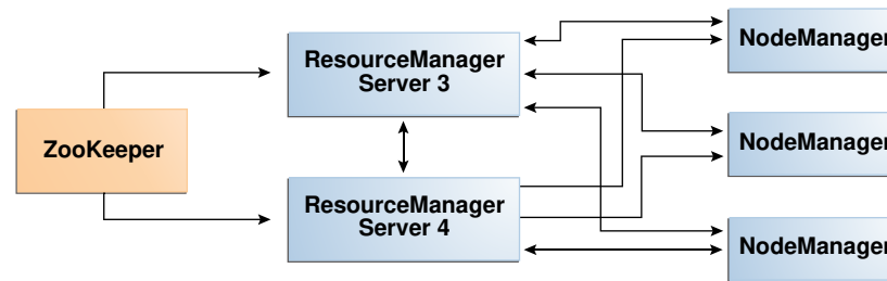
Figure 3-8 Automatic Failover of the ResourceManager on Oracle Big Data Appliance
