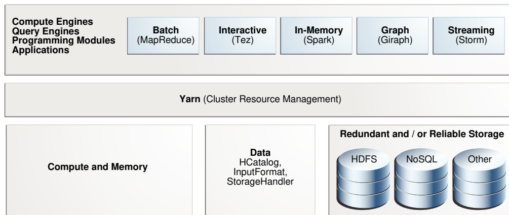
Figure 6-1 Hadoop 2.0 Architecture
