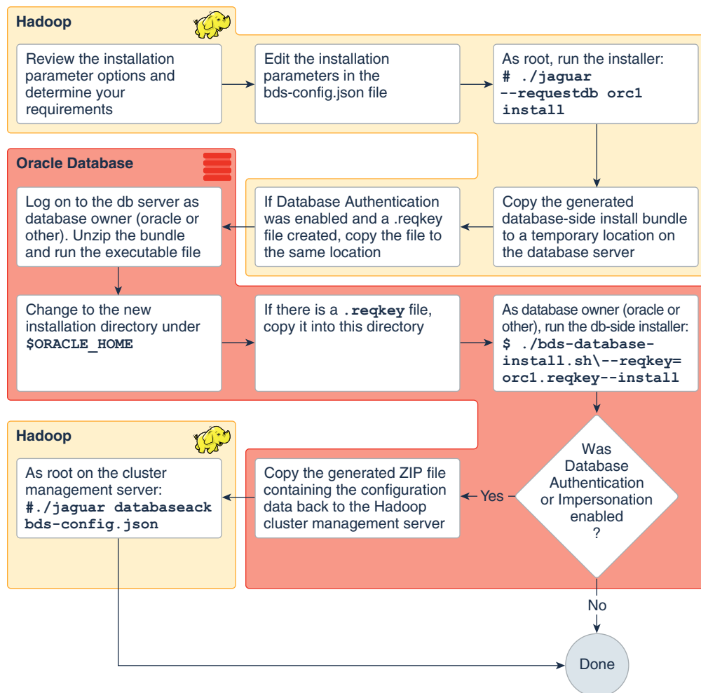
Figure 1-1 Installation Workflow
