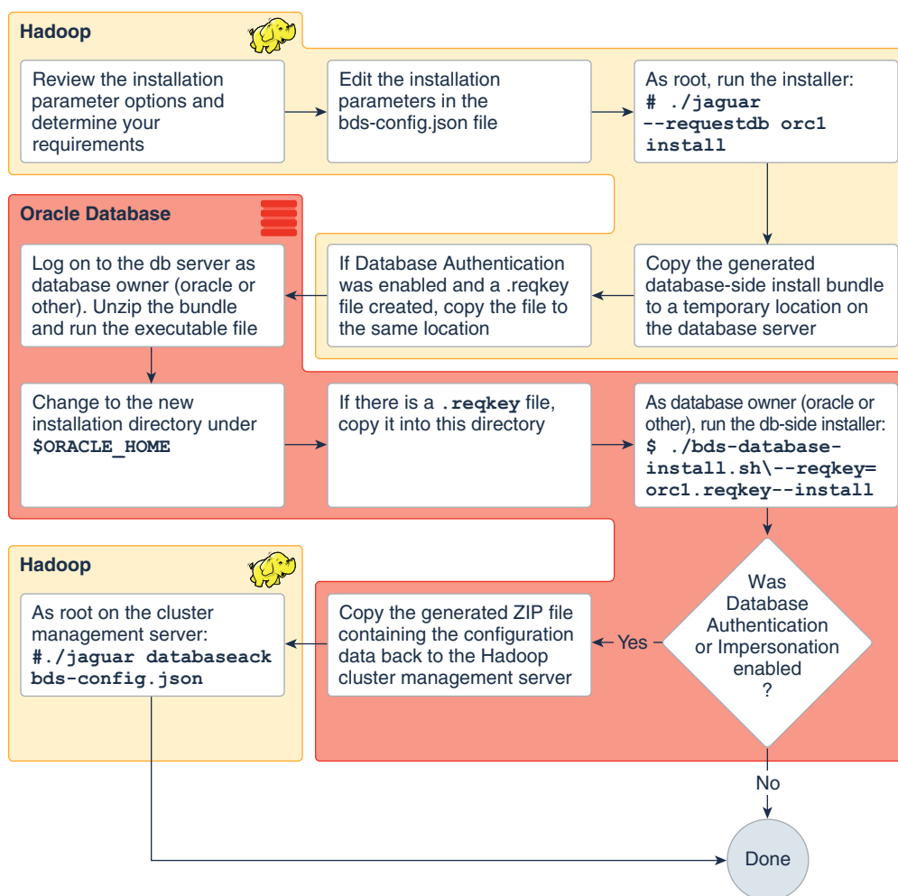
Figure 1-1 Installation Workflow
