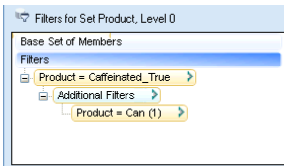
Figure 16-2 Intersection of Sets
