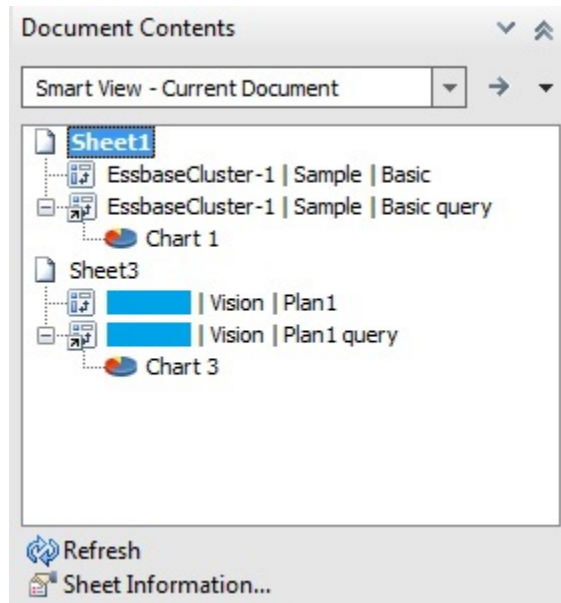
Figure 14-7 An Essbase Ad Hoc Grid with the Sheet Node Selected in Document Contents
