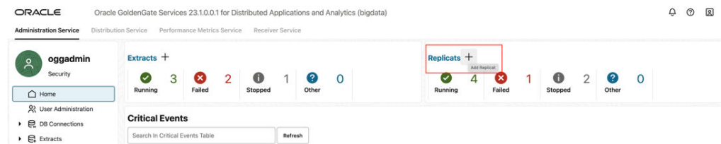
Figure 8-28 Administration Service
