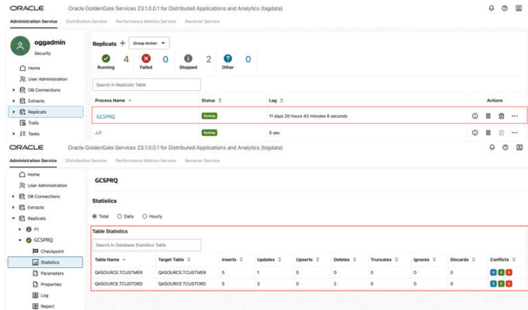
Figure 8-25 Replicats Statistics
