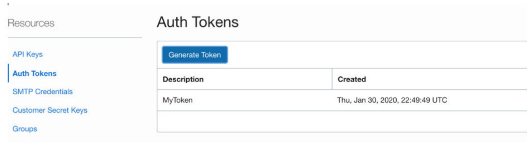
Figure 9-6 Auth-Tokens
