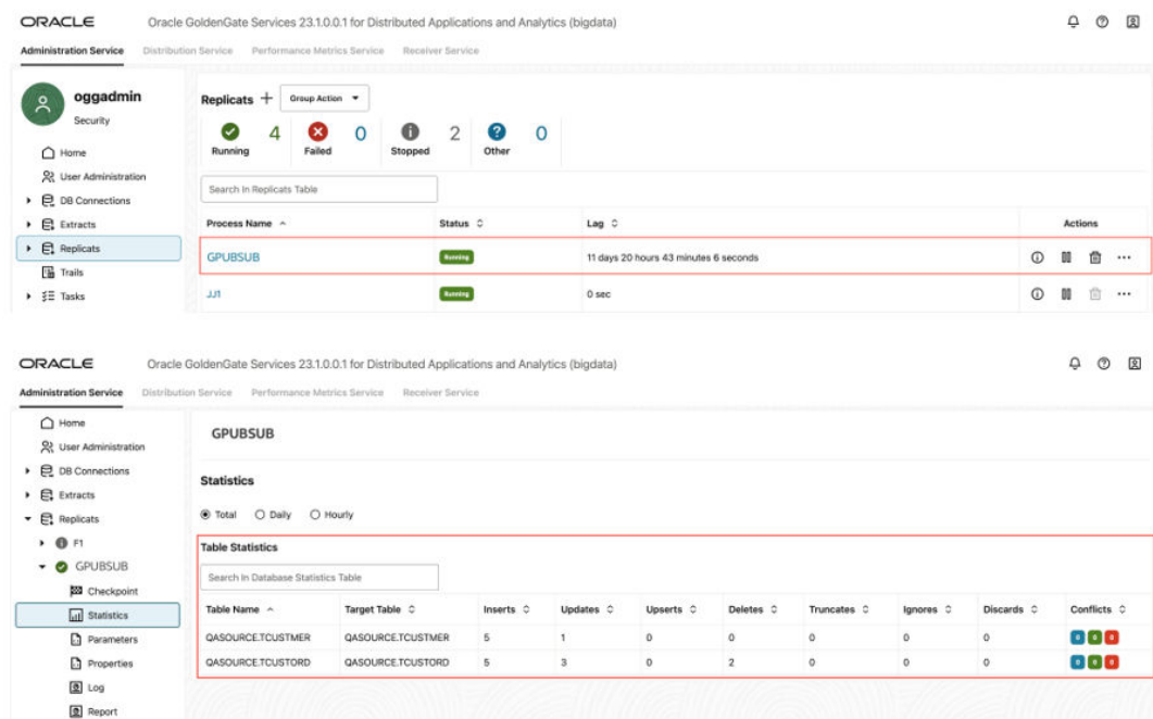
Figure 8-106 Replication Statistics
