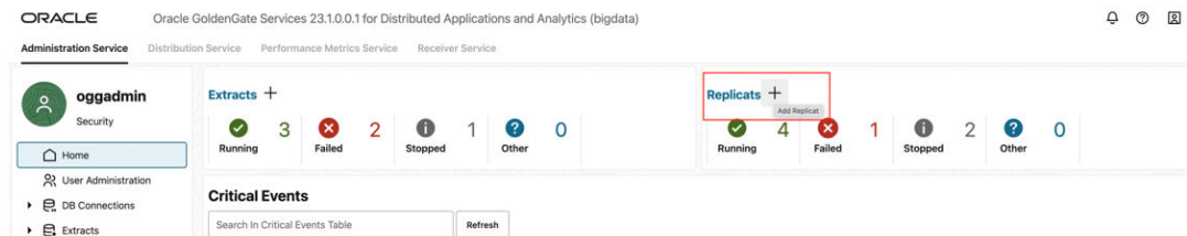
Figure 8-12 Administration Service
