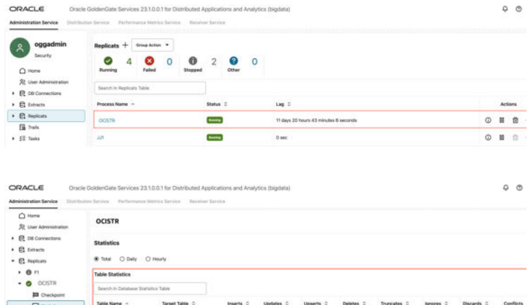
Figure 8-81 Replicat Statistics
