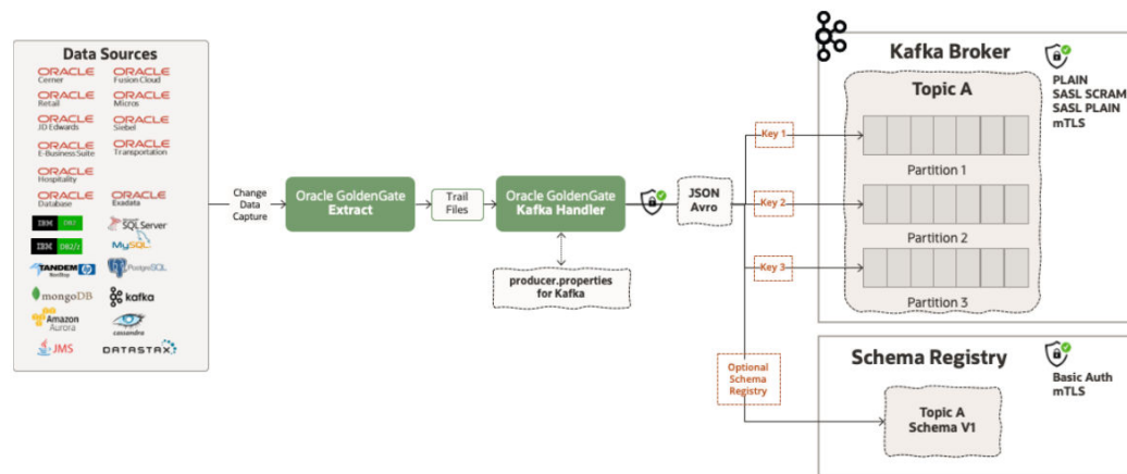
Figure 9-1 Apache Kafka Replication Architecture
