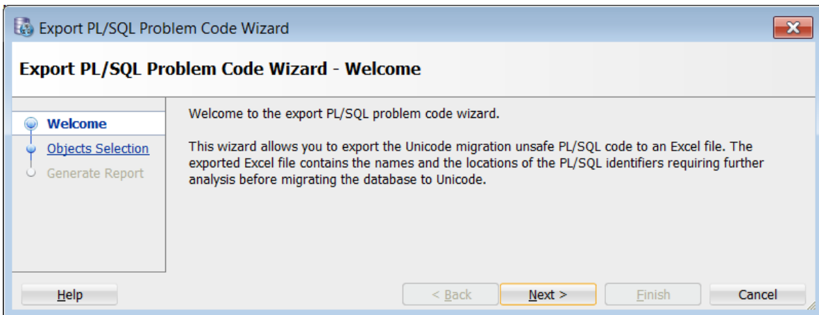
Figure 4-28 Export PL/SQL Problem Code Wizard - Welcome Page
