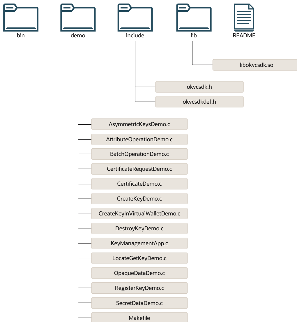
Figure 4-6 C SDK Directories and Files
