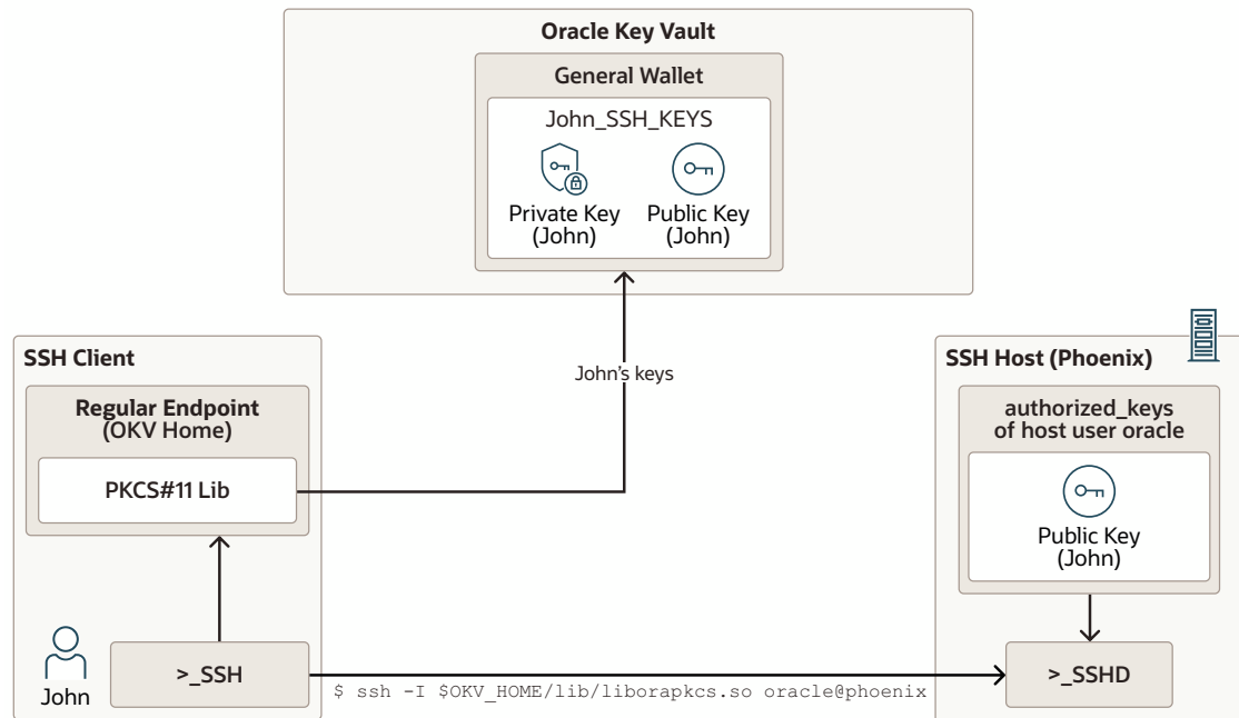
Figure 15-6 Centralized-SSH-User-Key-Management
