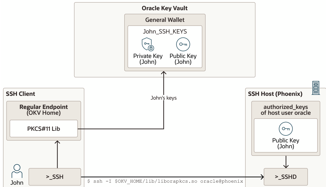
Figure 15-7 Centralized-SSH-Key-Management
