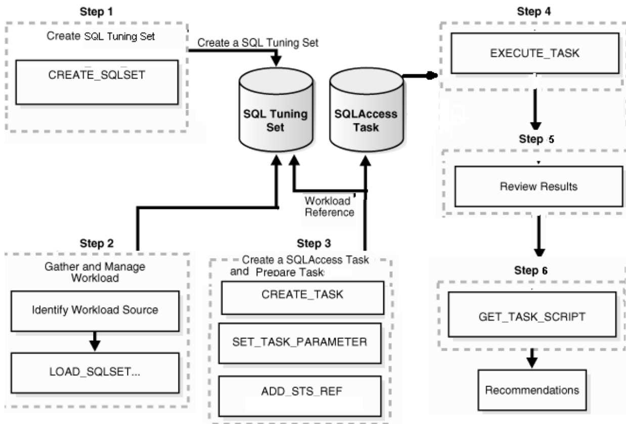
Figure 26-3 Using SQL Access Advisor
