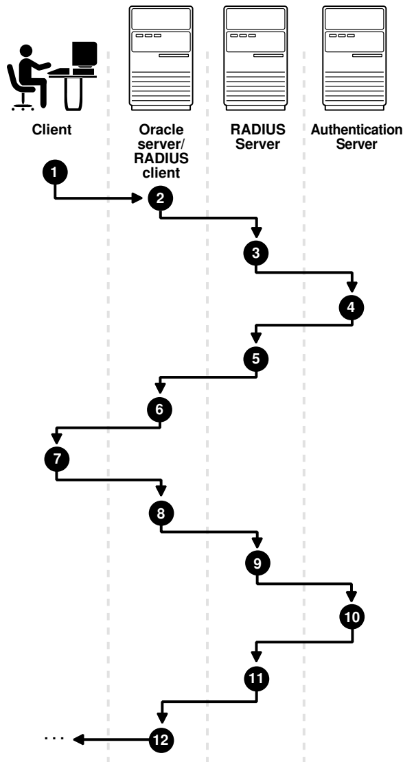
Figure 21-3 Asynchronous Authentication Sequence
