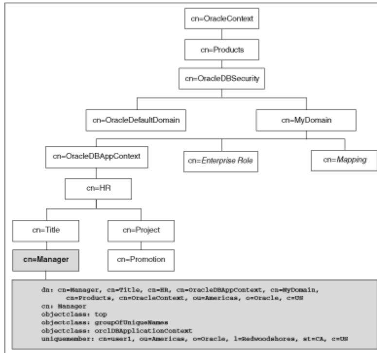
Figure 10-1 Location of Application Context in LDAP Directory Information Tree
