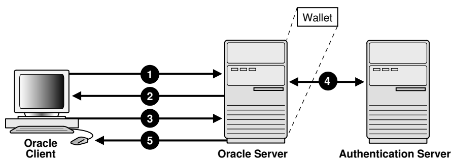
Figure 20-1 Secure Sockets Layer in Relation to Other Authentication Methods
