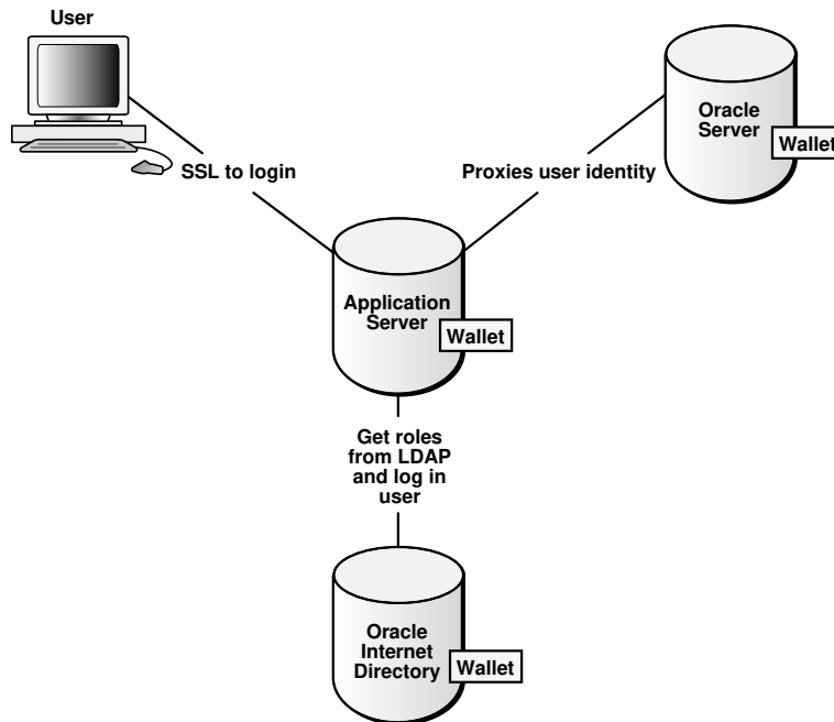
Figure 3-2 Multitier Authentication
