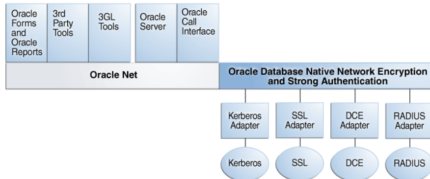
Figure 17-4 Oracle Net Services with Authentication Adapters
