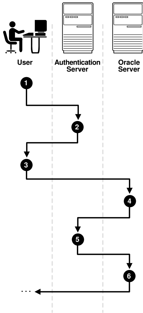
Figure 17-2 How a Network Authentication Service Authenticates a User
