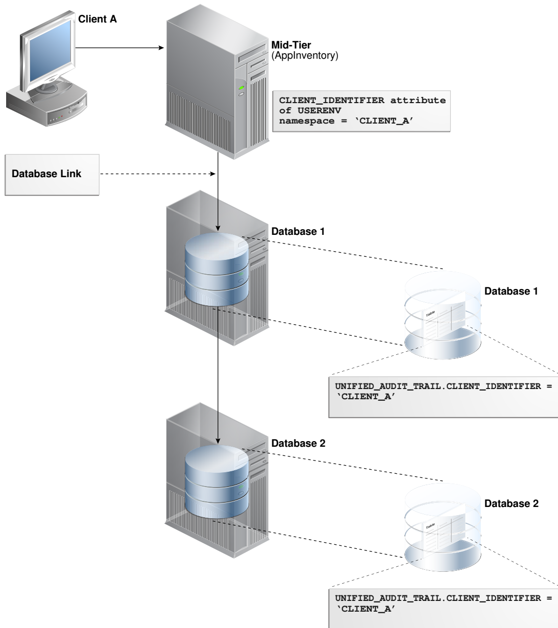
Figure 24-2 Auditing Client Identifier Information Across Sessions
