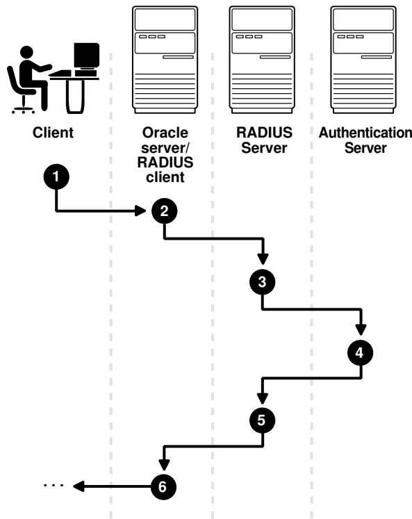
Figure 21-2 Synchronous Authentication Sequence
