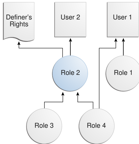
Figure 6-3 Roles Granted to Application Users and Definer's Rights Program Unit
