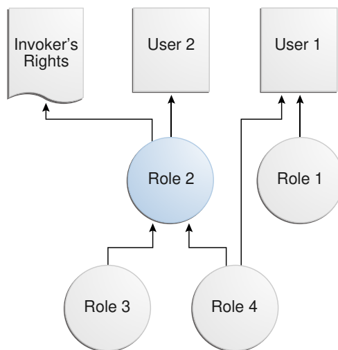
Figure 6-1 Roles Granted to Application Users and Invoker's Right Program Unit
