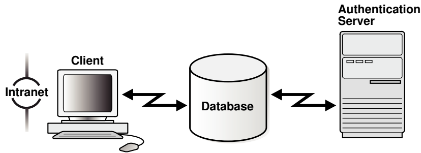
Figure 17-1 Strong Authentication with Oracle Authentication Adapters
