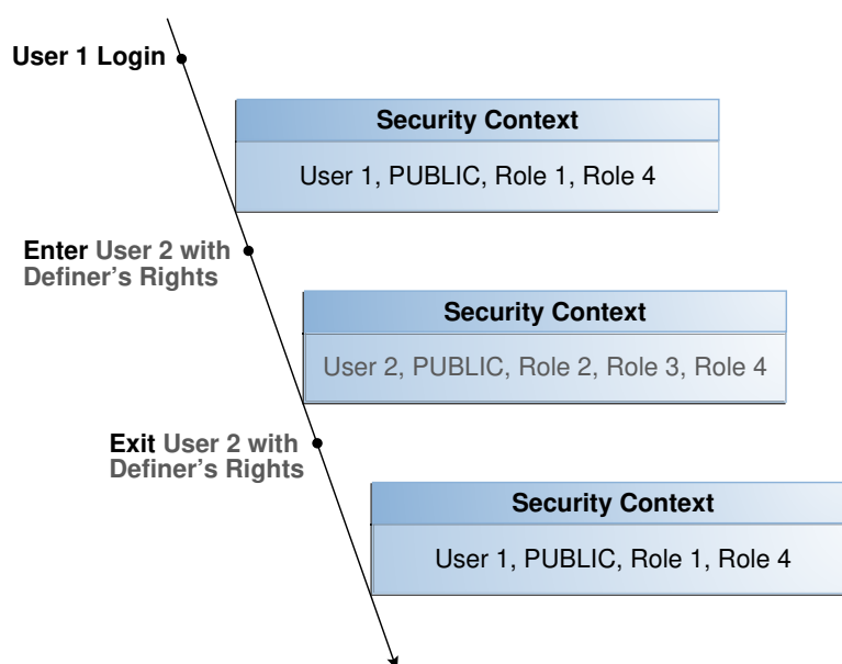
Figure 6-4 Security Context in Which Definer's Right Program Unit DR Is Executed
