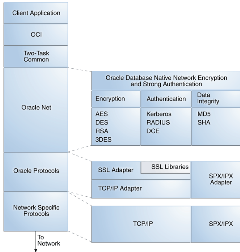
Figure 17-3 Oracle Native Network Encryption and Strong Authentication Architecture
