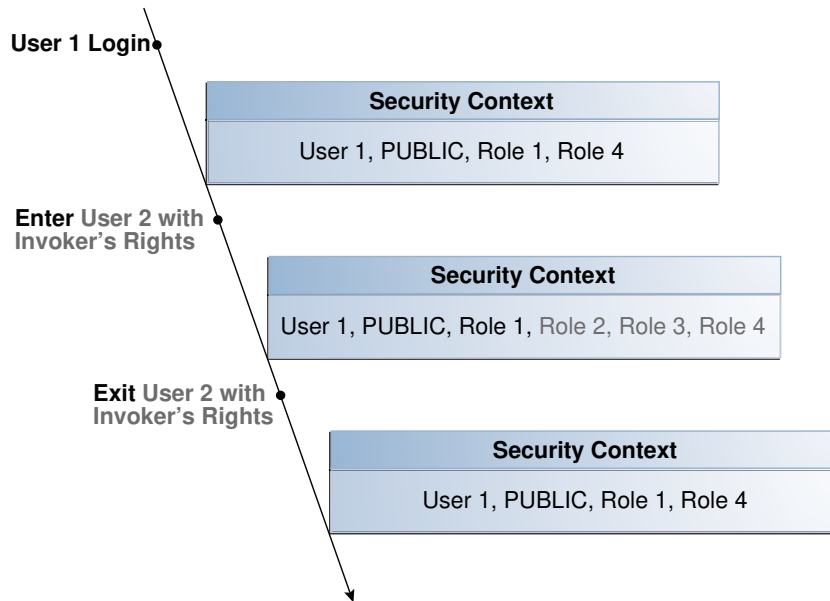
Figure 6-2 Security Context in Which Invoker's Right Program Unit IR Is Executed
