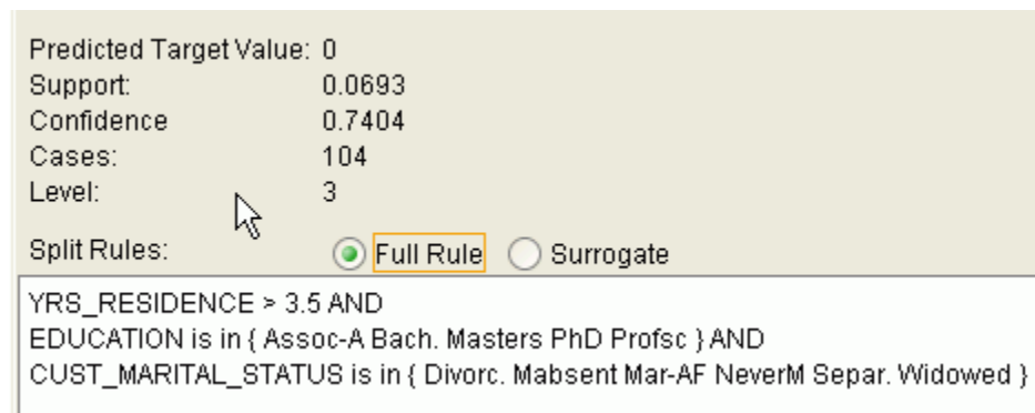
Figure 13-1 Sample Decision Tree Rule
