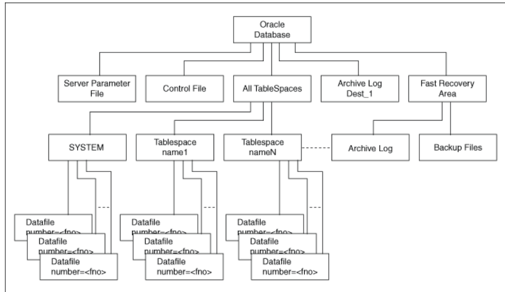
Figure 9-1 Oracle VSS Writer Component Hierarchy
