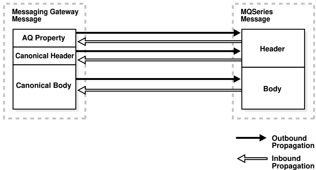
Figure 20-3 Message Conversion for WebSphere MQ Using MGW_BASIC_MSG_T
