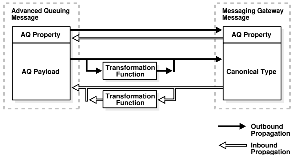
Figure 20-2 Oracle Database Advanced Queuing Message Conversion
