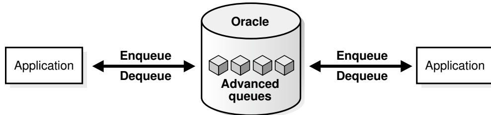
Figure 1-6 Point-to-Point Messaging
