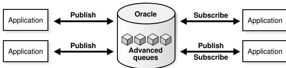
Figure 1-7 Publish/Subscribe Mode
