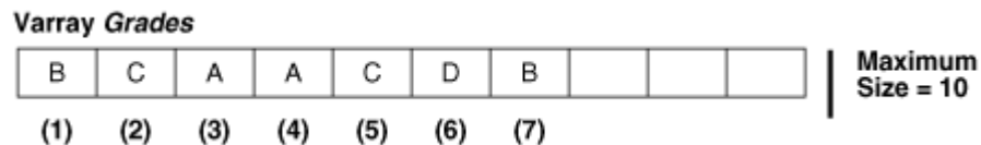
Figure 5-1 Varray of Maximum Size 10 with 7 Elements
