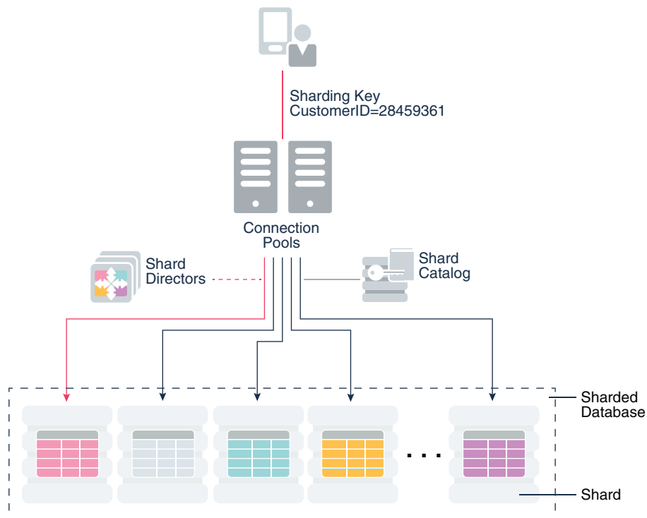
Figure 11-1 Oracle Sharding Architecture
