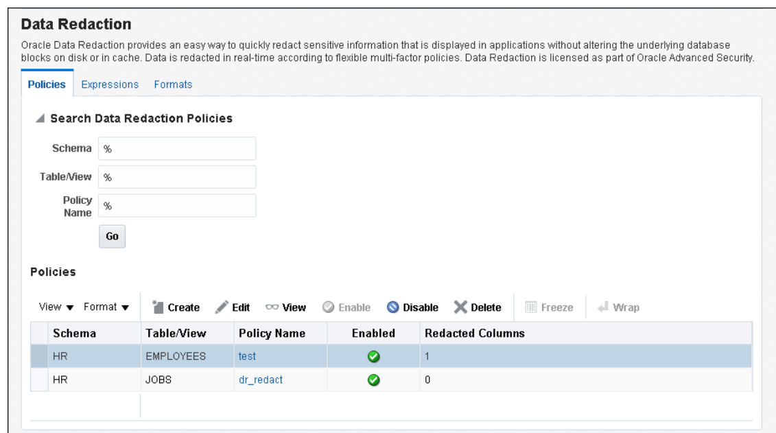
Figure 17-4 Oracle Data Redaction Policies Page
