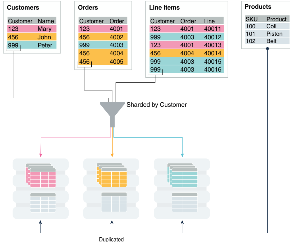
Figure 2-4 Horizontal Partitioning of a Table Across Shards
