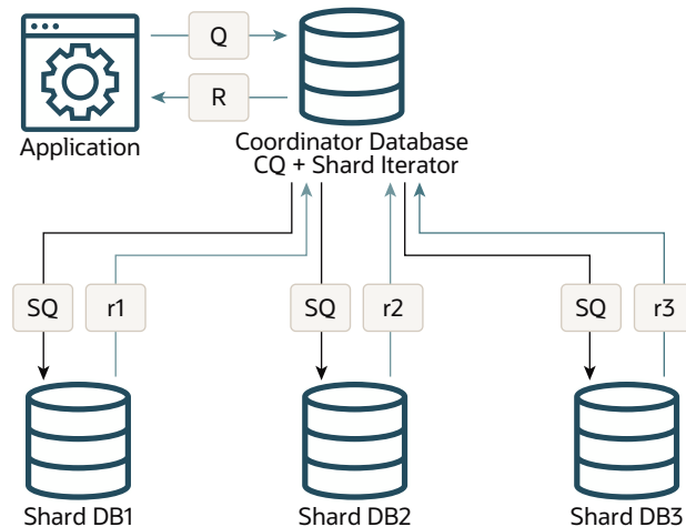
Figure 9-3 Query Coordinator Operation
