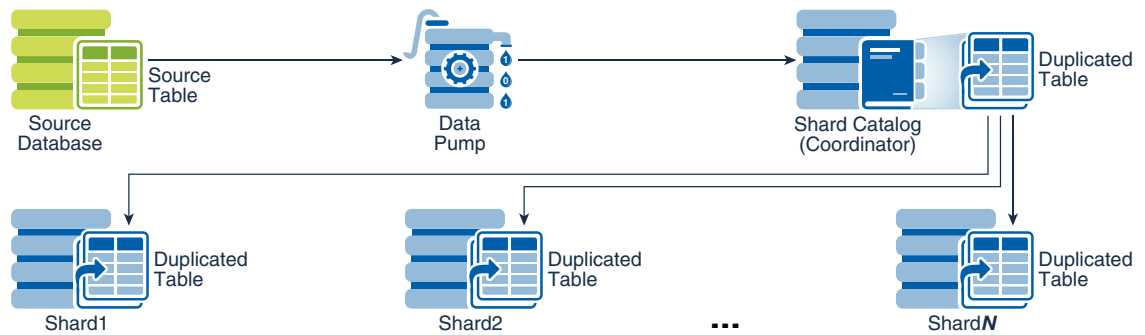
Figure 8-2 Loading Duplicated Tables
