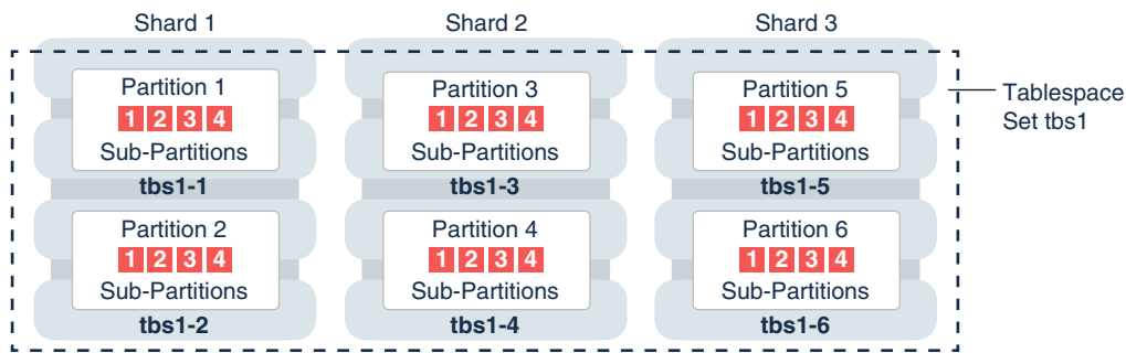
Figure 2-10 Subpartitions Stored in the Tablespace of the Parent Partition
