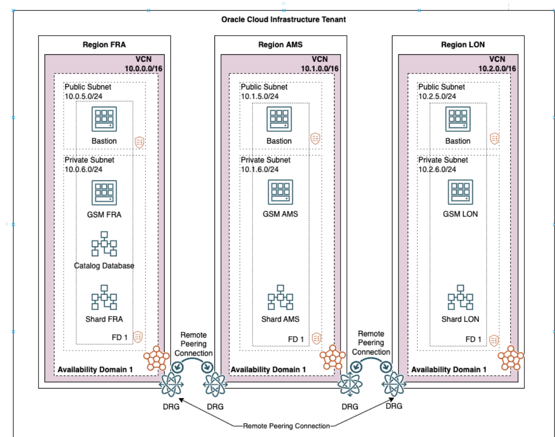
Figure 13-3 Deployment Topology of Data Sovereignty with Oracle Sharding
