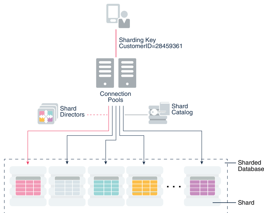
Figure 13-1 Oracle Sharding Architecture
