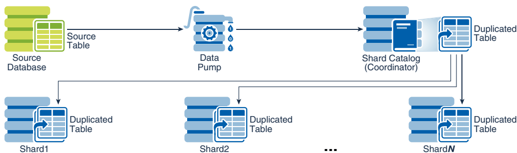
Figure 8-2 Loading Duplicated Tables
