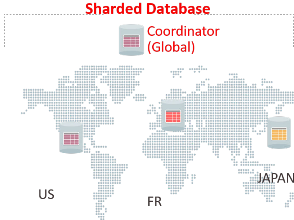
Figure 13-2 Sharded Database
