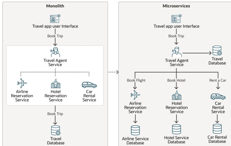
Figure 26-1 Monolith and Microservices
