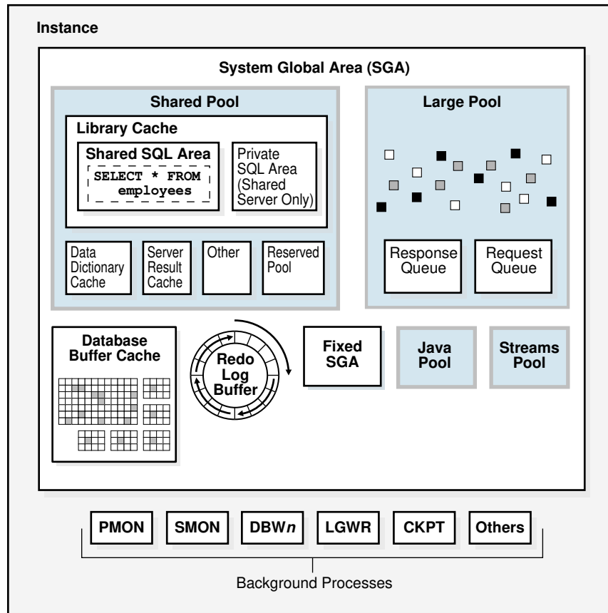
Figure 16-1 Database Instance
