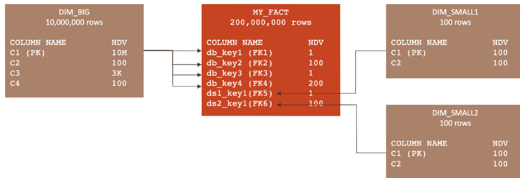
Figure 12-8 Candidate Dimension Table for Semi-Join Materialized View Rewrite
