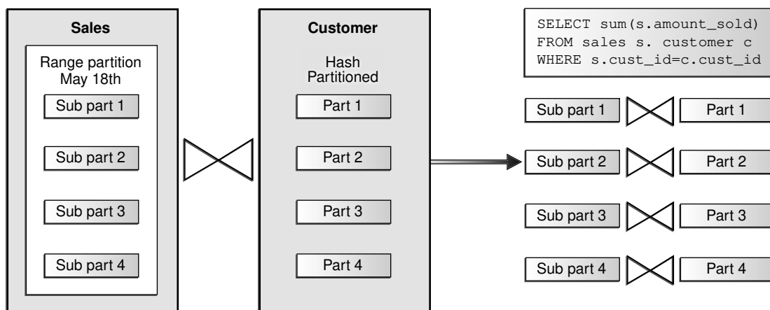
Figure 4-4 Full Partition-Wise Join
