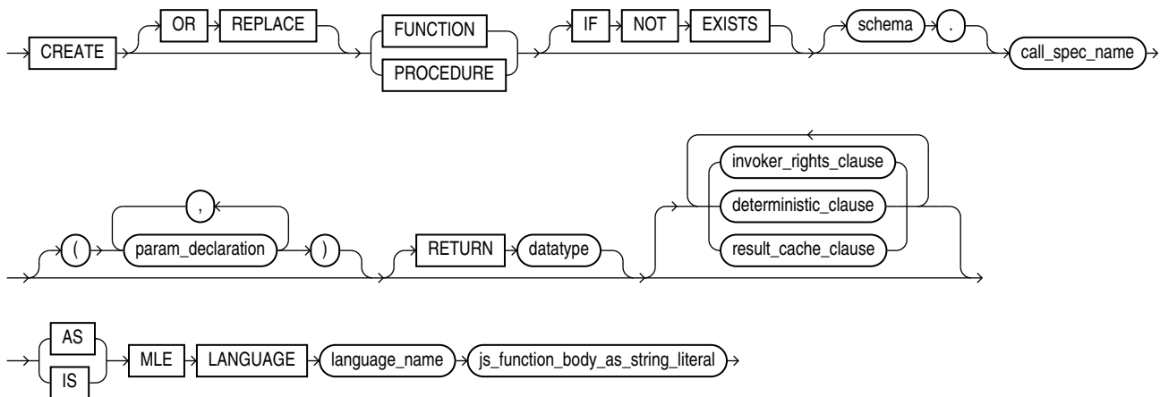
Figure 5-2 MLE Inlined Call Specification Syntax
