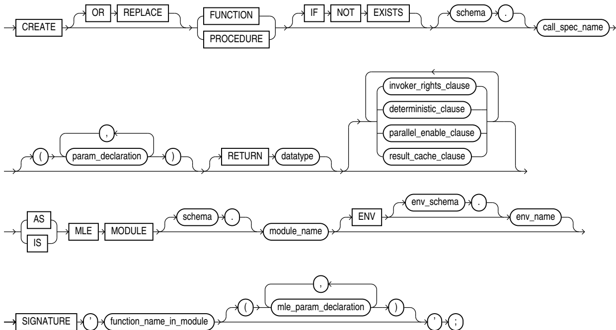
Figure 5-1 MLE Call Specification Syntax
