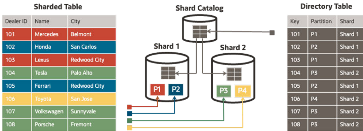
Figure 2-9 Directory-based sharding architecture
