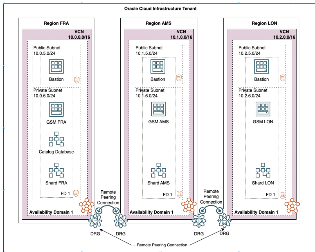
Figure 16-3 Deployment Topology of Data Sovereignty
