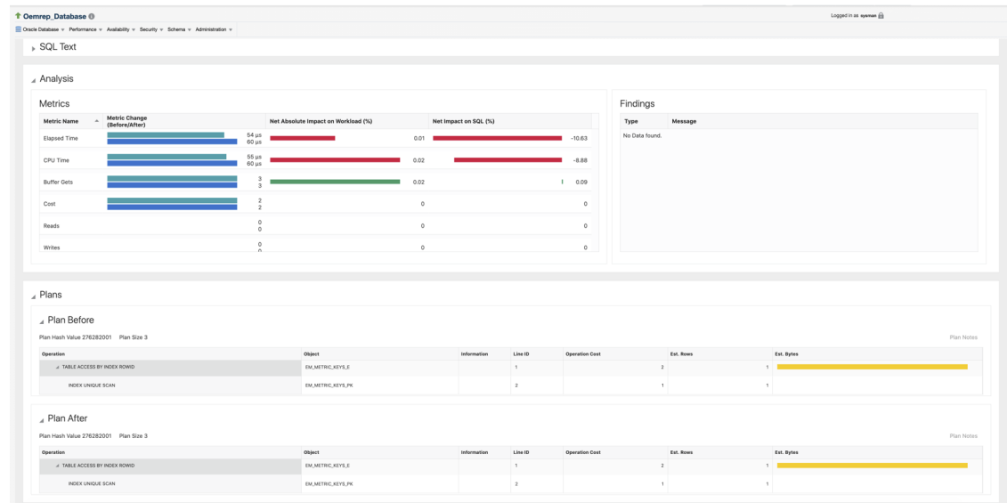
Figure 17-5 SQL Details
