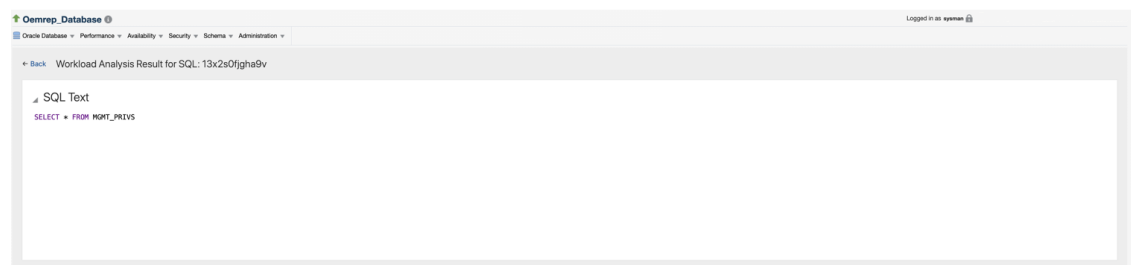
Figure 17-6 SQL Text
