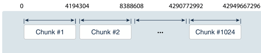
Figure 2-6 Ranges of Hash Values Assigned to Chunks
