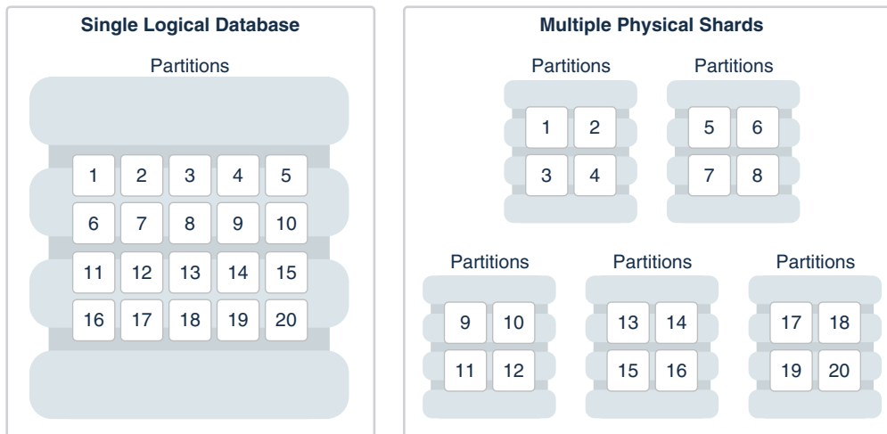
Figure 1-2 Oracle Globally Distributed AI Database as Distributed Partitioning
