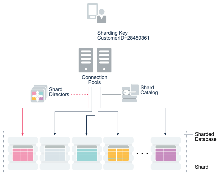
Figure 2-1 Oracle Globally Distributed AI Database Architecture
