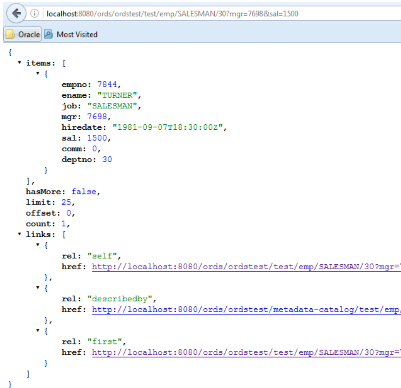
Figure 3-10 Using Browser to Show the Results of Using a Query String to Send a GET Method with Some Parameter Name/Value Pairs
