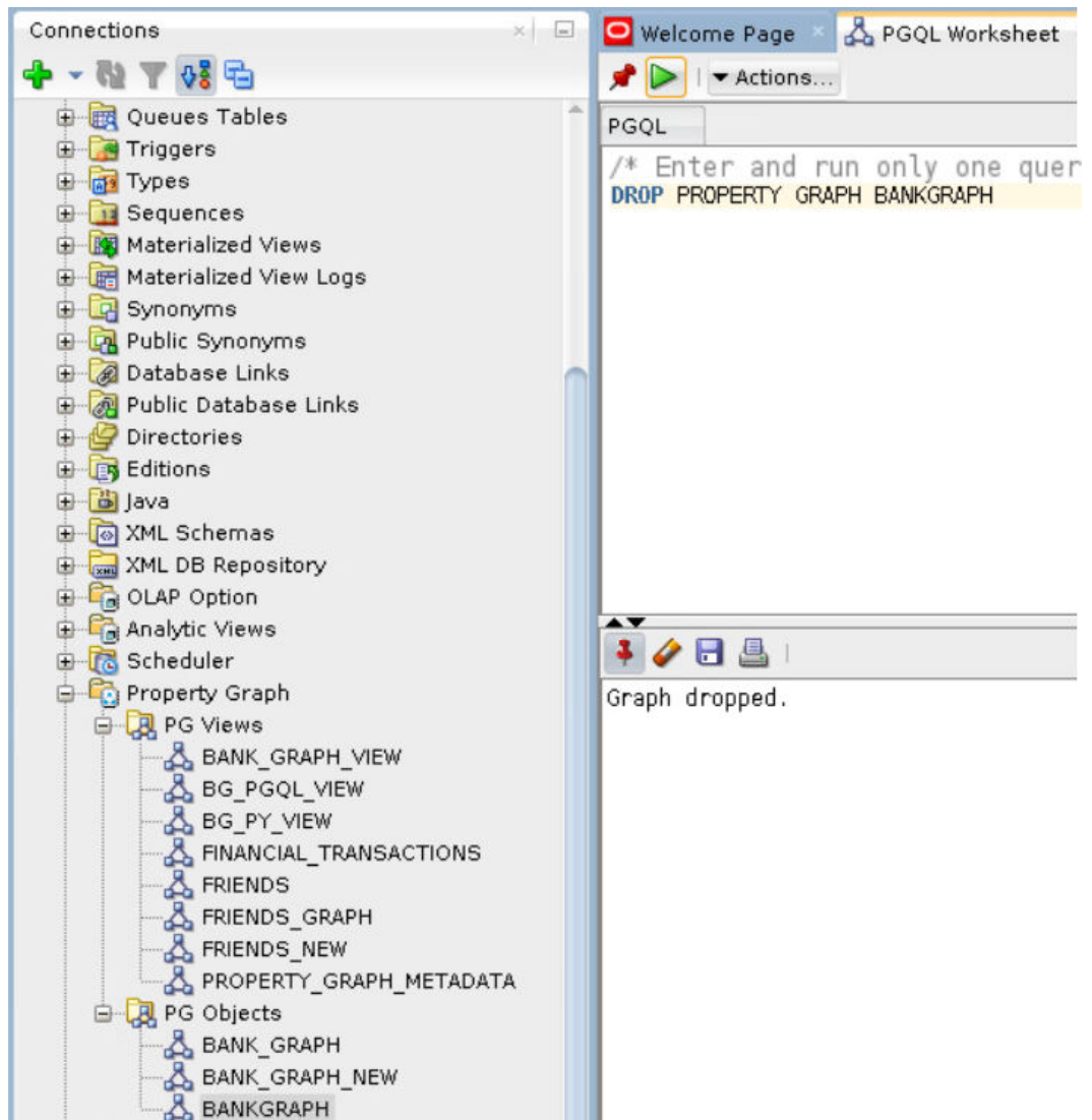
Figure 6-11 Dropping a Property Graph Object
