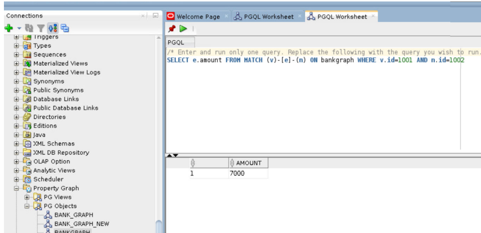
Figure 6-10 Running a PGQL SELECT Query
