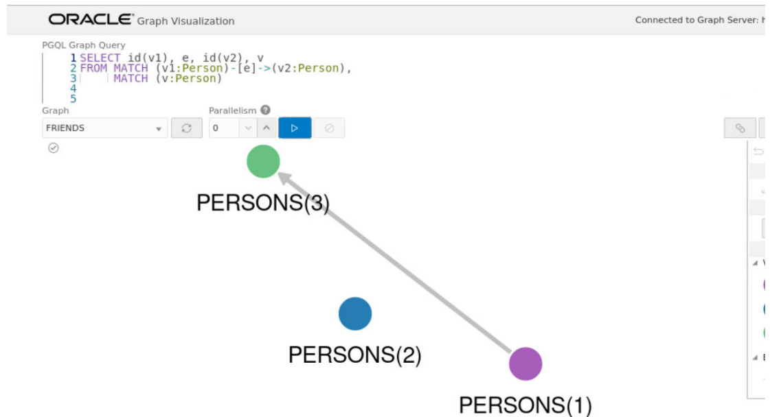
Figure 3-2 Subgraph Visualization
