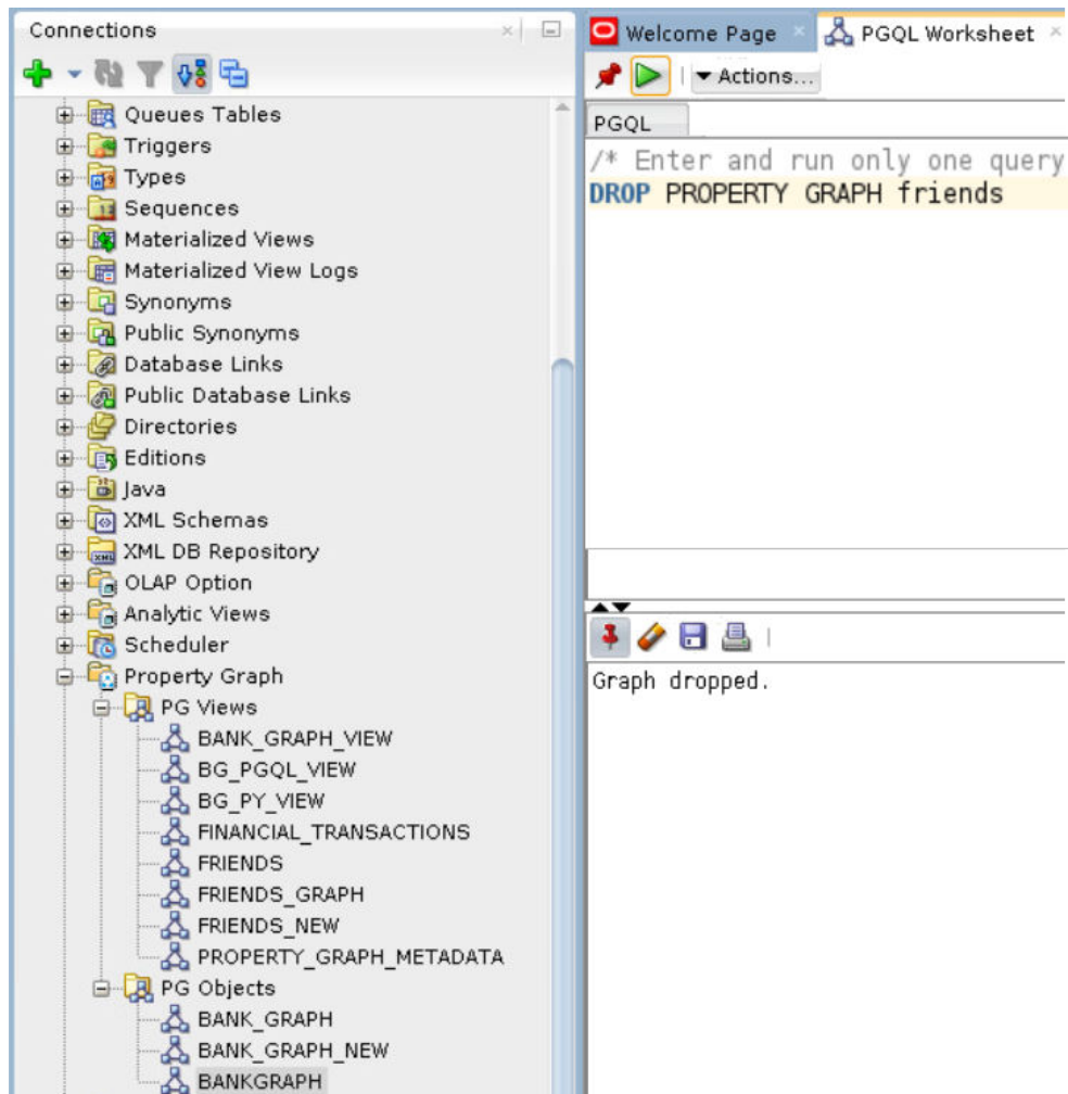
Figure 6-7 Dropping a Property Graph View
