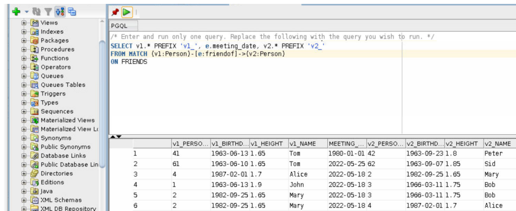
Figure 6-6 Running a PGQL SELECT Query
