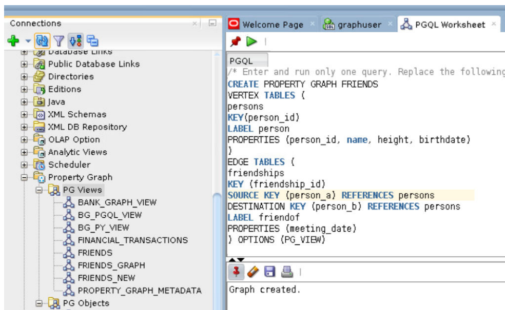
Figure 6-4 Create a Property Graph View
