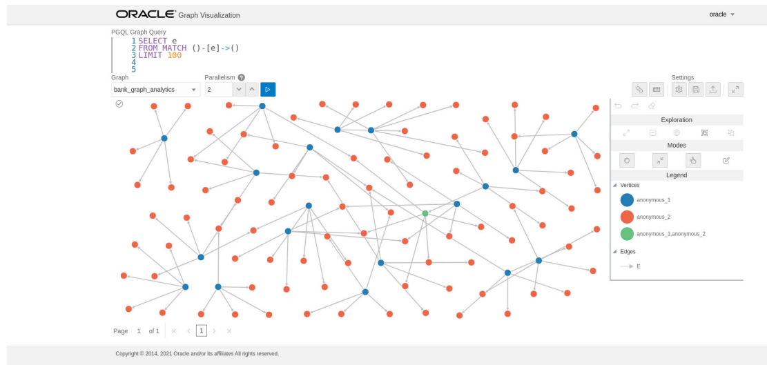
Figure 7-1 Query Visualization
