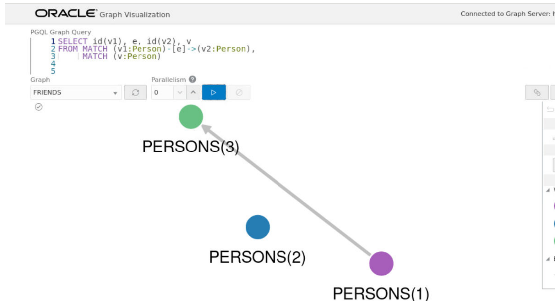
Figure 3-2 Subgraph Visualization
