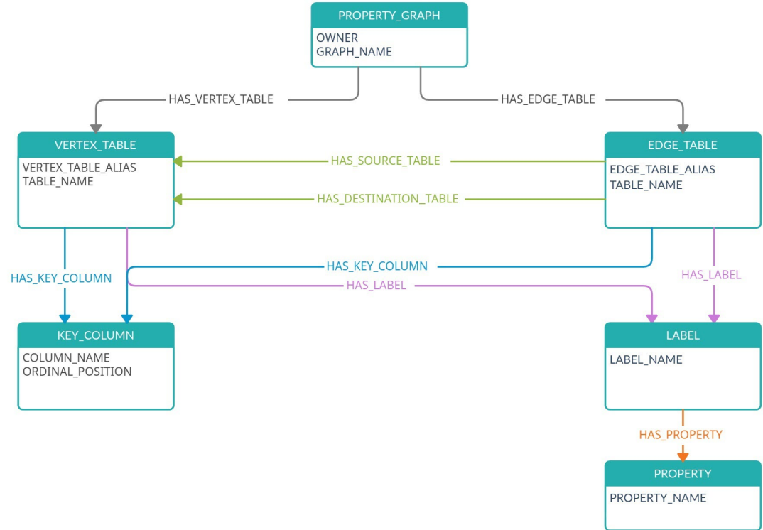
Figure 3-4 PROPERTY_GRAPH_METADATA Graph Design
