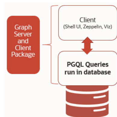
Figure 1-3 Two-Tier Property Graph Architecture
