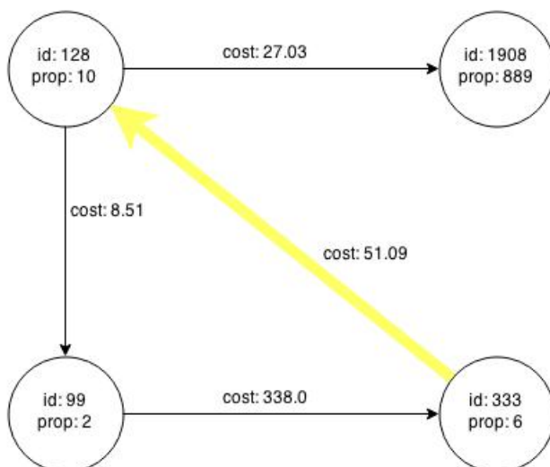
Figure 16-3 Edges Matching the outDegree Filter
