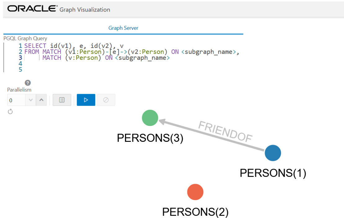
Figure 10-1 Subgraph Visualization
