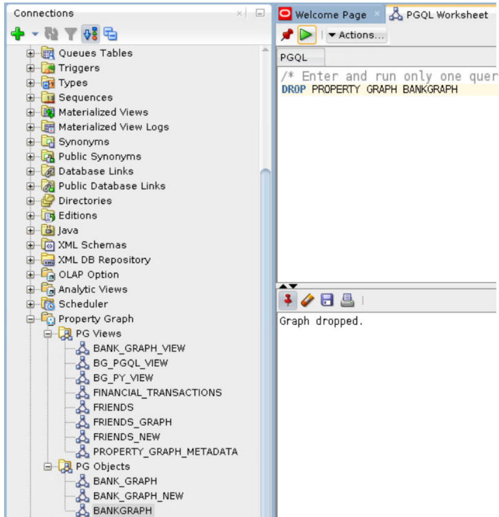
Figure A-5 Dropping a Property Graph Object
