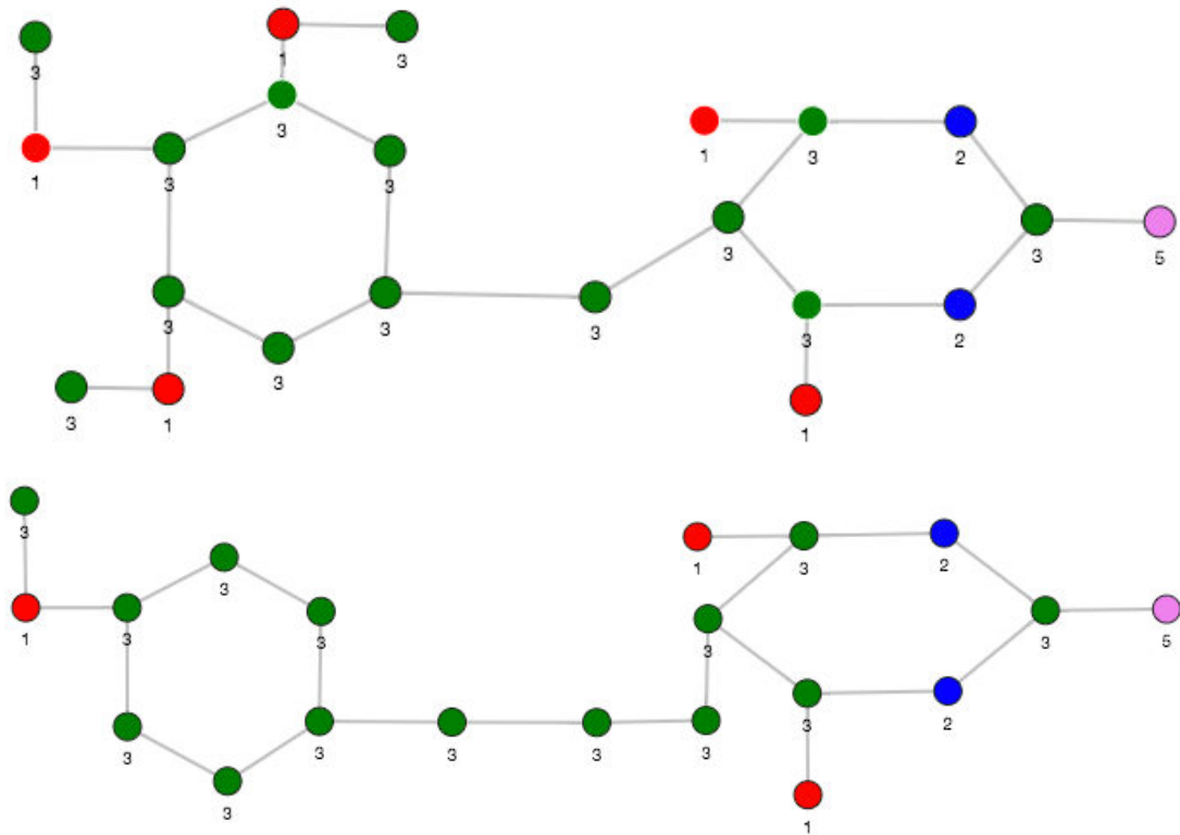
Figure 17-1 Pg2vec - Visualization of Two Similar Graphlets
