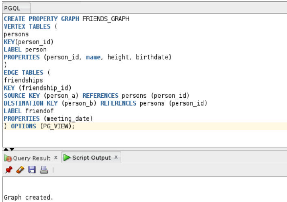
Figure 12-4 Create a PGQL property graph
