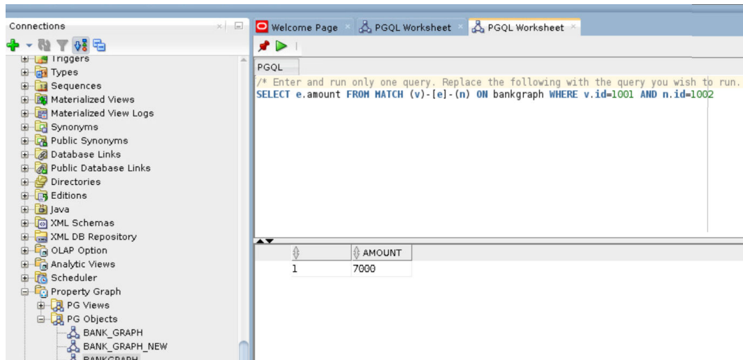
Figure A-4 Running a PGQL SELECT Query
