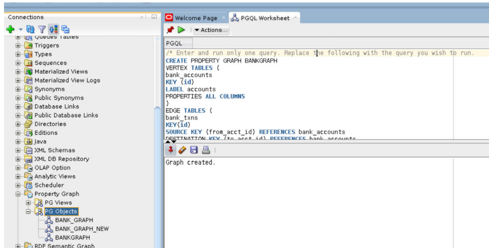
Figure A-2 Creating a Property Graph Object
