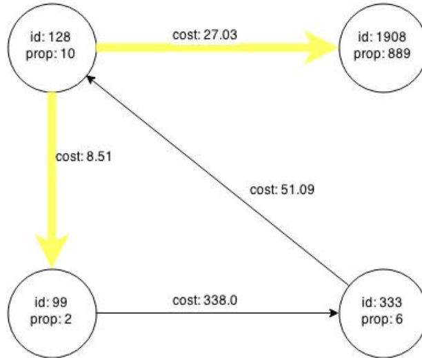
Figure 16-1 Edges Matching src.prop == 10
