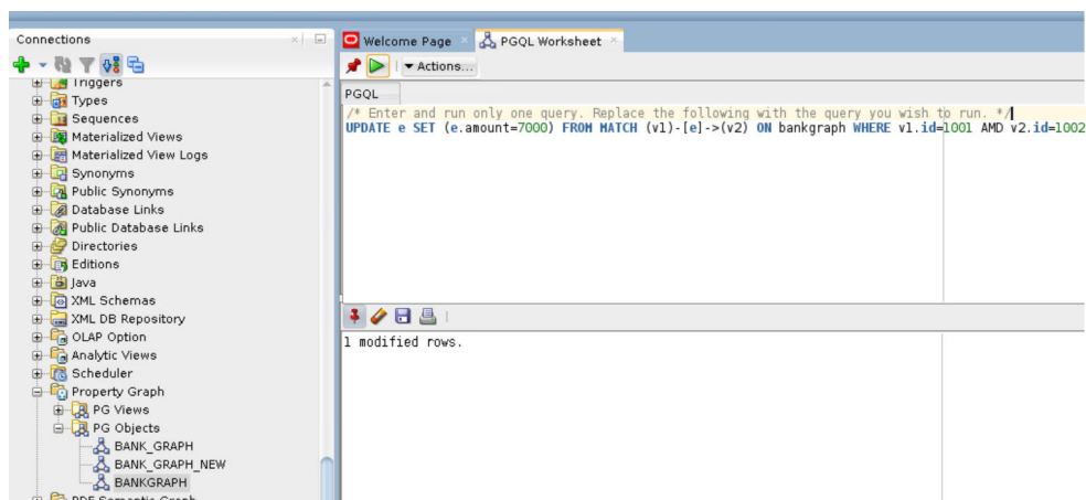
Figure A-3 Updating a Property Graph Object
