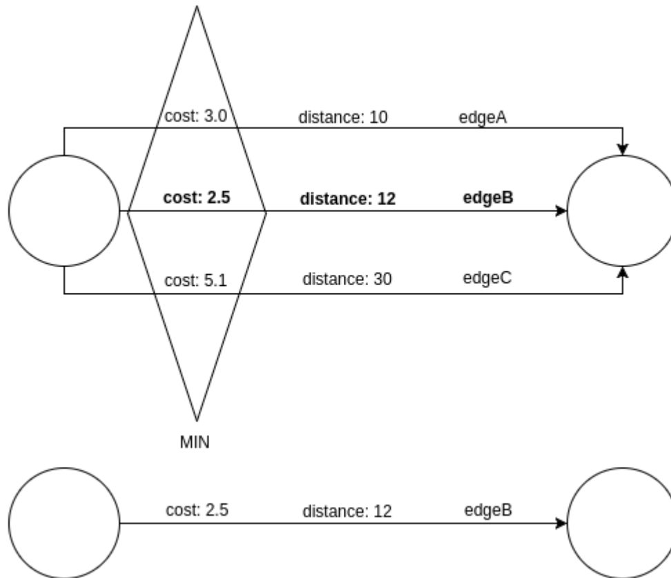
Figure 26-1 Picking Strategy
