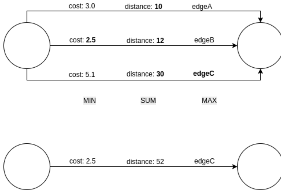
Figure 26-2 Merging Strategy
