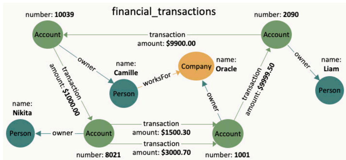
Figure 9-2 Financial Transactions Graph
