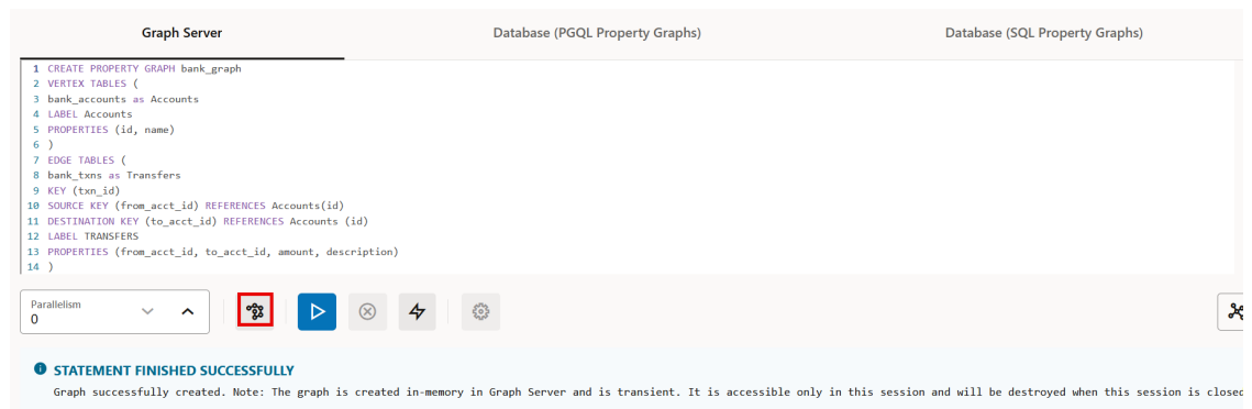
Figure 21-3 Creating a Property Graph in the Graph Server Memory
