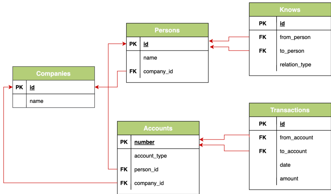
Figure 13-1 Example Schema
