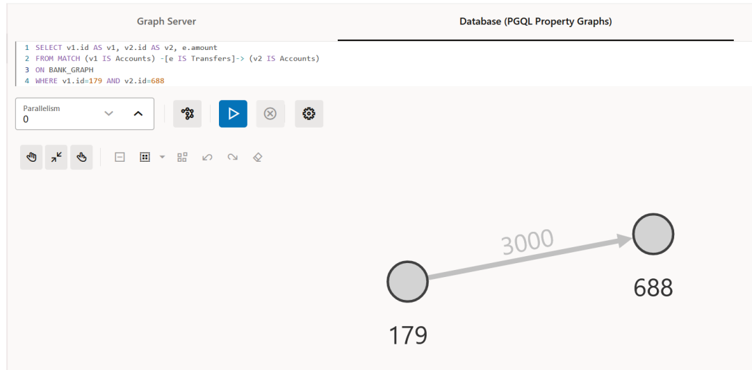
Figure 21-10 Querying a PGQL property graph
