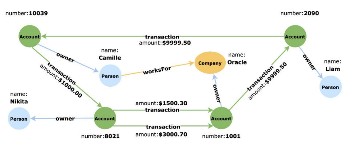
Figure 13-3 Financial_Transactions Graph
