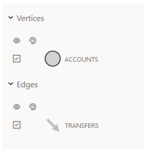
Figure 21-14 Graph Legend
