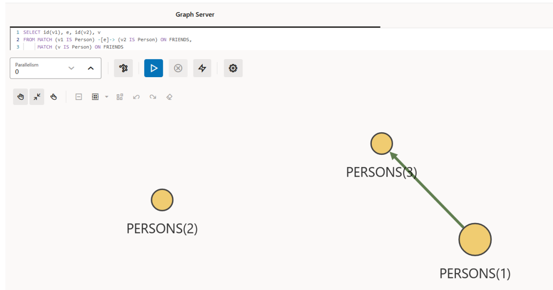
Figure 10-1 Subgraph Visualization
