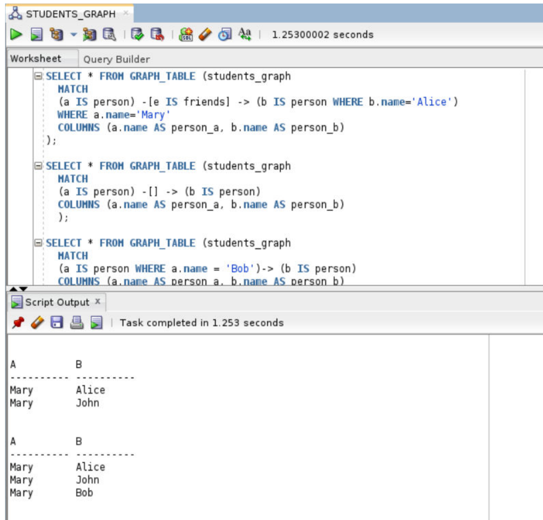
Figure 5-2 Running SQL Graph queries in SQL Developer
