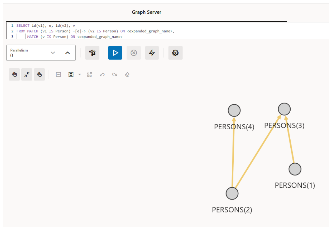
Figure 10-2 Expanding a Subgraph
