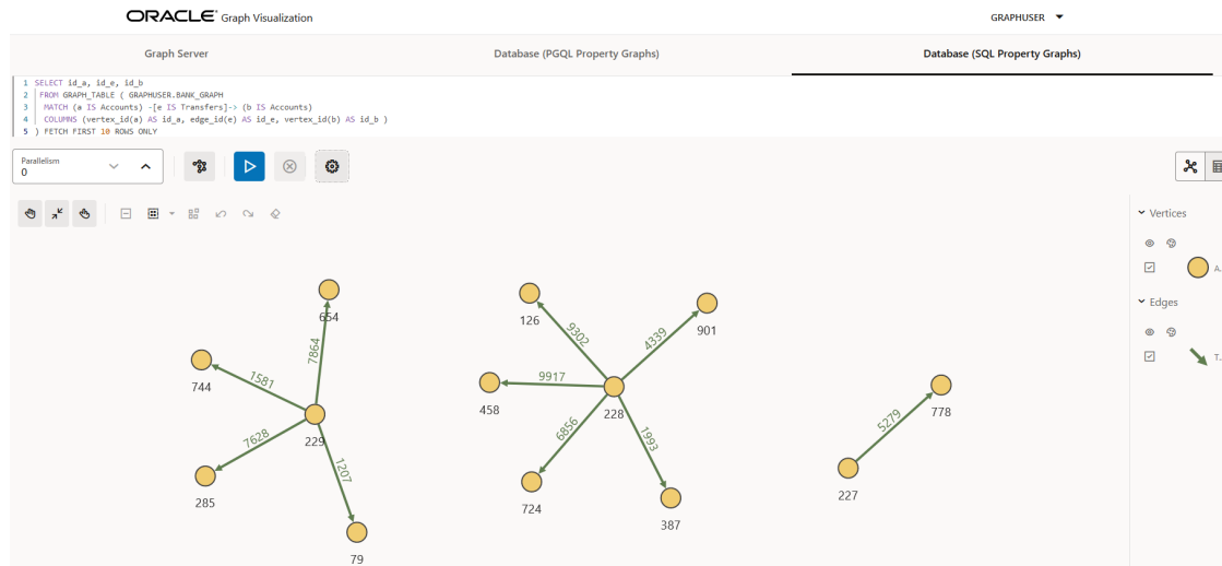
Figure 21-12 Graph Query on a SQL Property Graph
