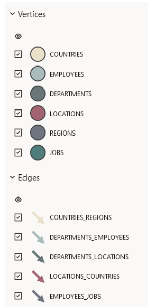
Figure 21-14 Graph Legends
