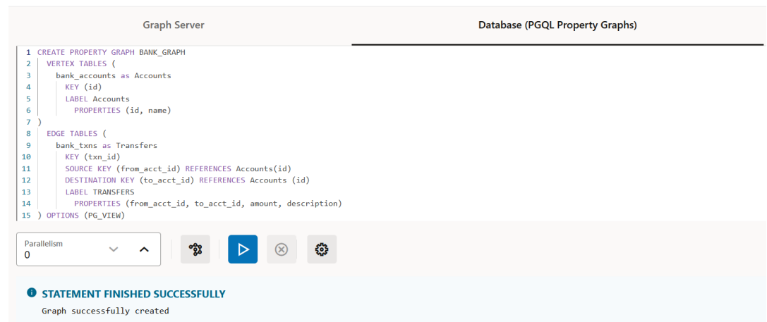
Figure 21-7 Creating a PGQL property graph
