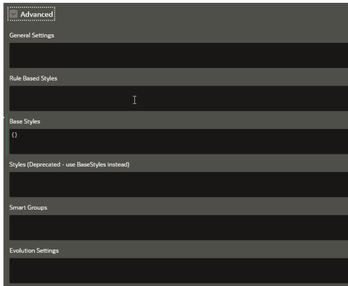
Figure 8-7 Advanced Options
