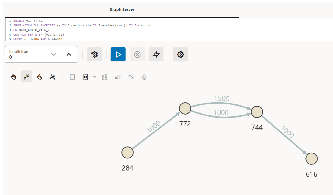
Figure 20-1 Visualizing Unnesting of Variable-Length Path Queries
