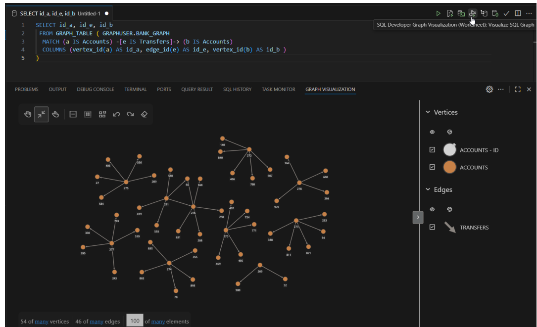
Figure 10-1 Graph Visualization of SQL Graph Queries in VS Code
