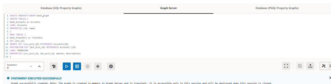
Figure 23-6 Creating a Property Graph in the Graph Server Memory
