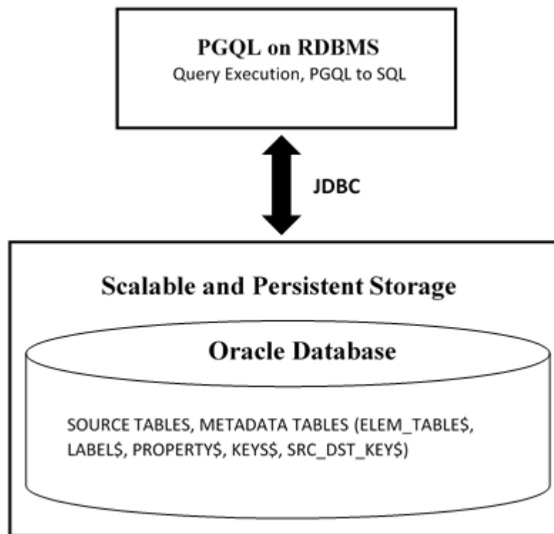
Figure 15-4 PGQL on PGQL Property Graphs in Database
