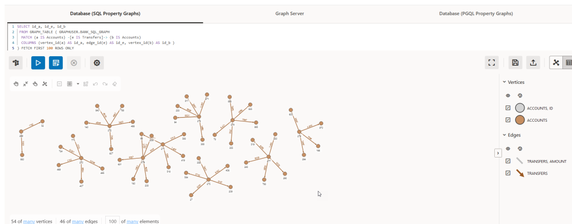
Figure 23-3 Graph Query on a SQL Property Graph
