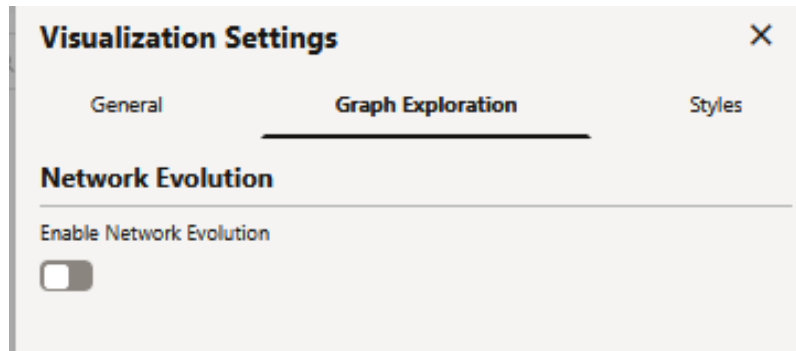
Figure 25-26 Graph Exploration
