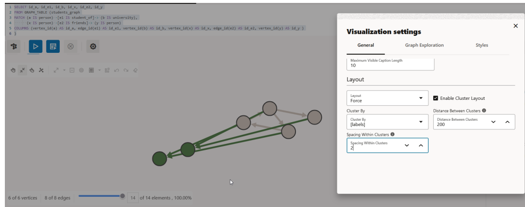
Figure 26-22 Cluster-Based Layout
