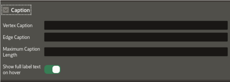
Figure 9-9 Captions
