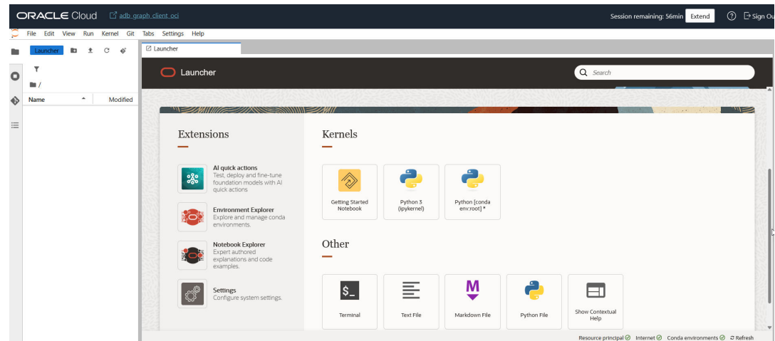
Figure 12-1 JupyterLab Interface
