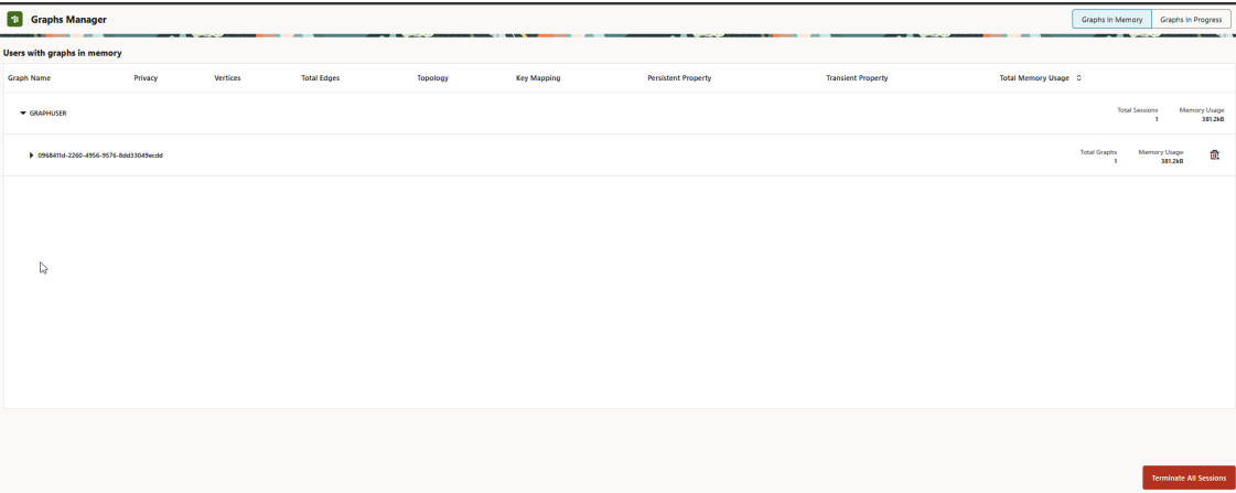
Figure 27-4 Graphs
