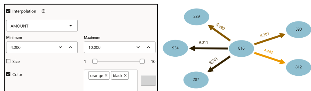
Figure 26-21 Interpolation in Graph Visualization
