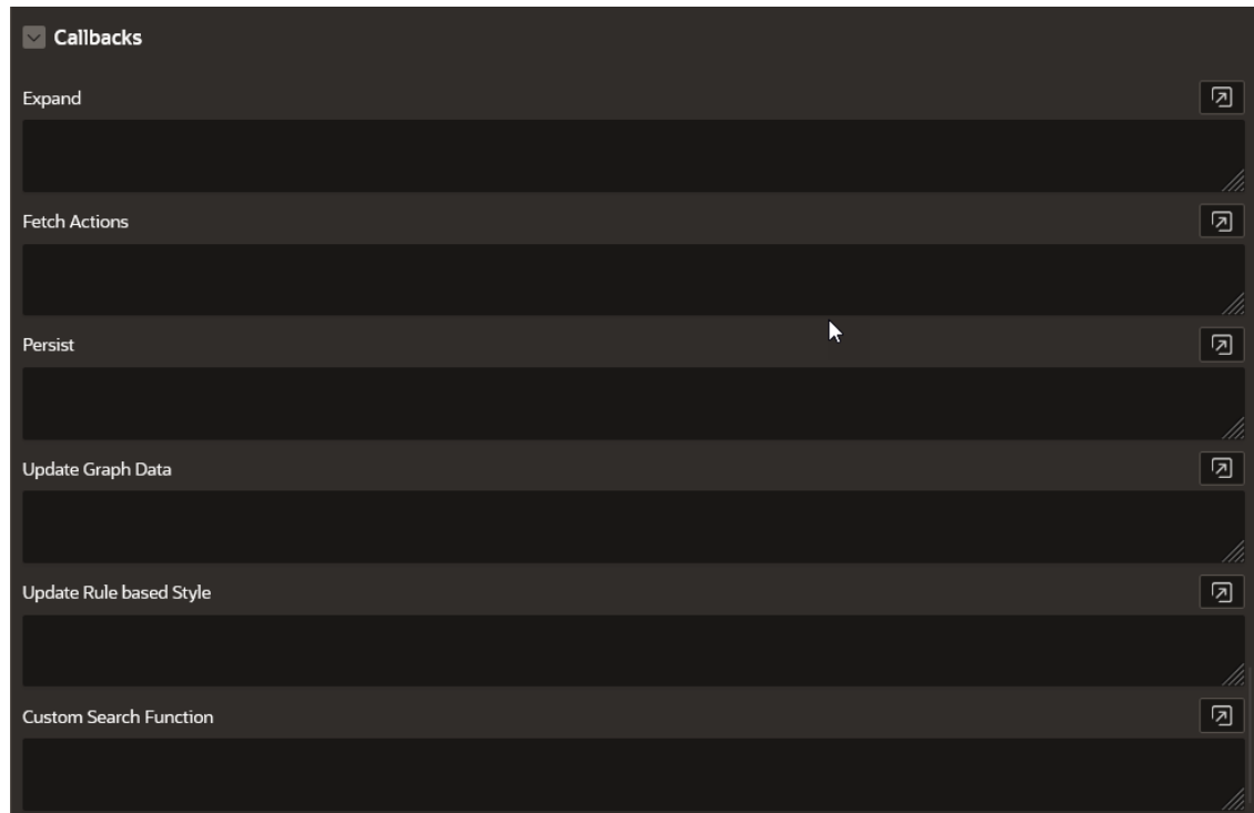
Figure 9-19 Callbacks
