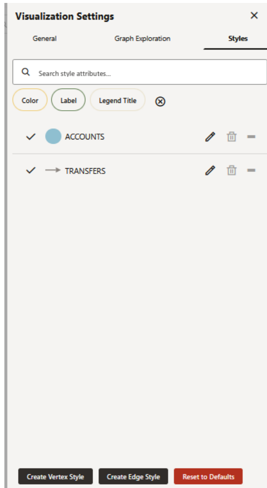
Figure 25-27 Styles Tab
