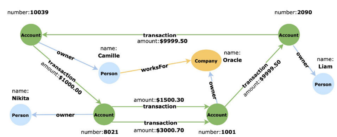
Figure 17-3 Financial_Transactions Graph
