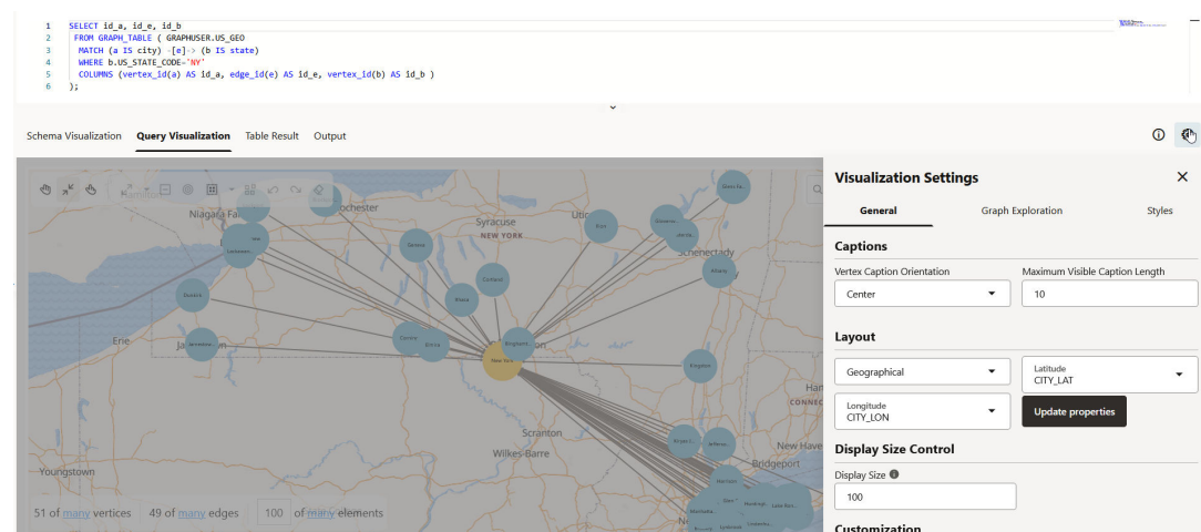
Figure 25-31 Geographical Layout
