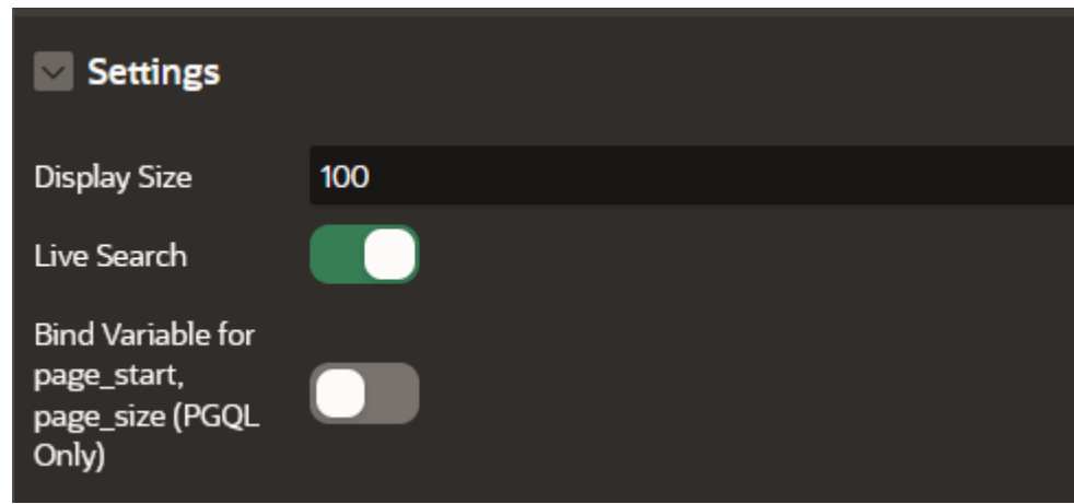
Figure 9-5 Settings
