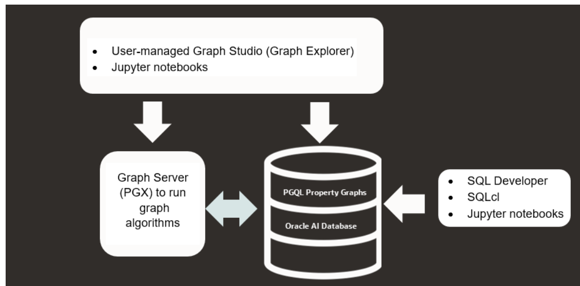
Figure 1-3 Tools for Querying, Visualizing, and Running Analytics on PGQL Property Graphs
