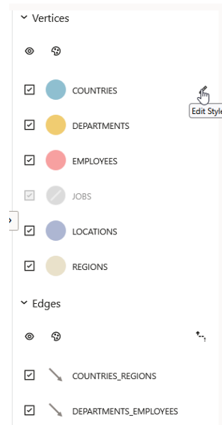
Figure 25-14 Graph Legends
