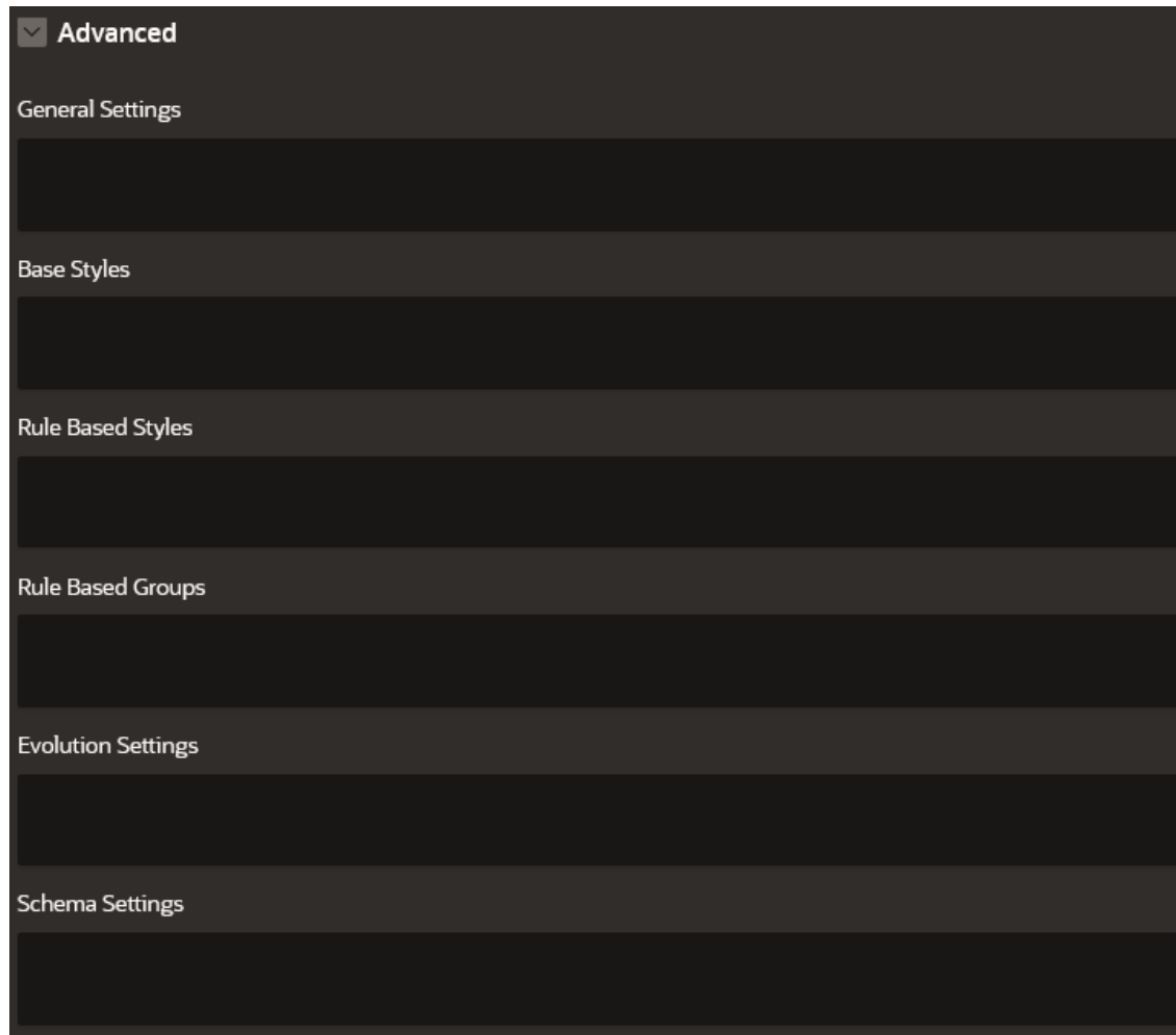
Figure 9-13 Advanced Options
