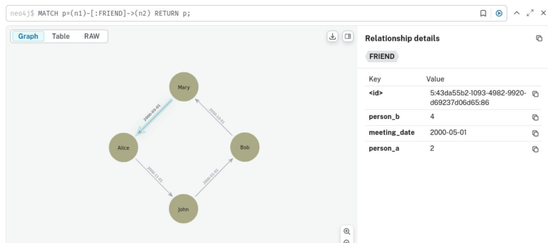
Figure 4-3 Example Graph in Neo4j for Migration
