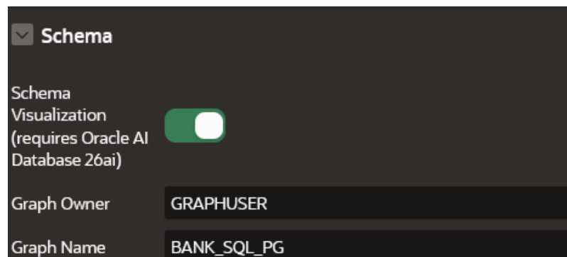
Figure 9-11 Schema
