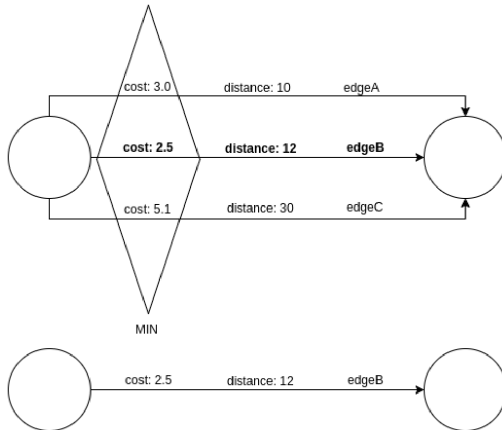
Figure 32-1 Picking Strategy
