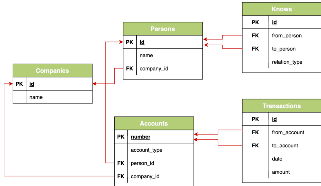
Figure 17-1 Example Schema
