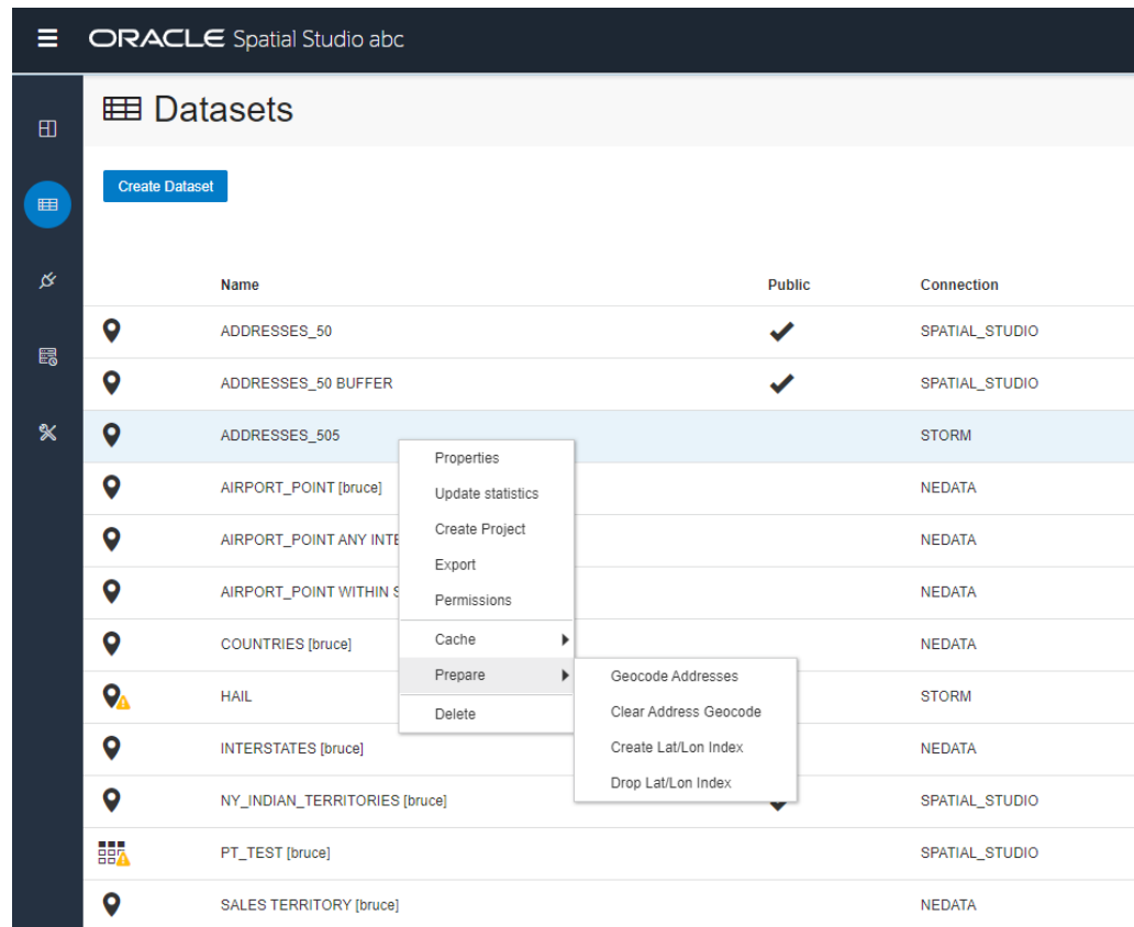
Figure 3-5 Data Page, Including Dropdown Menus
