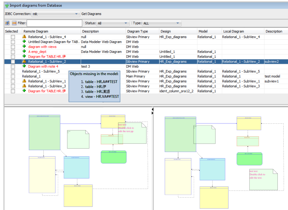
Figure 1-2 Import Diagrams from SQL Developer Web
