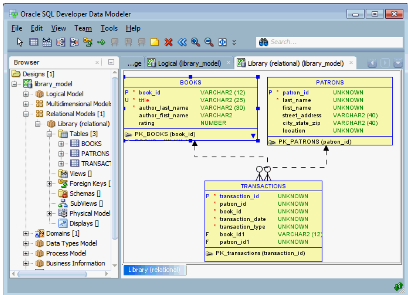
Figure 1-1 SQL Developer Data Modeler Main Window
