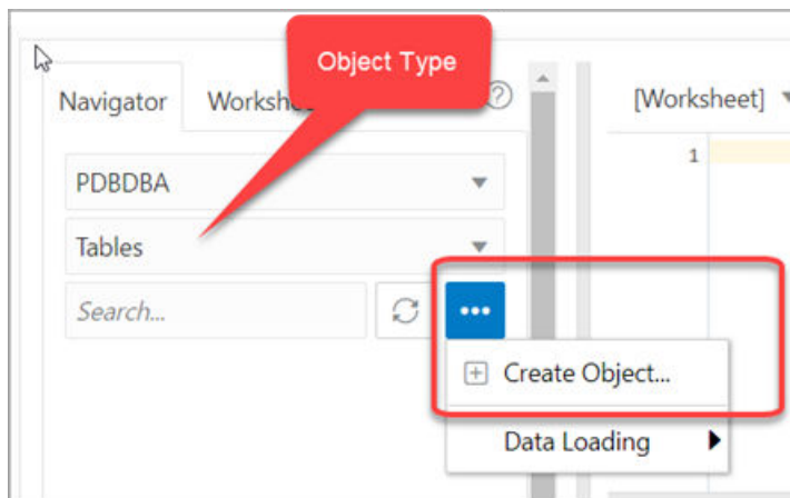
Figure 3-15 Create Object
