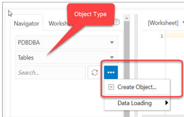
Figure 3-14 Create Object
