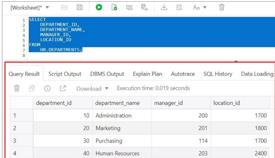
Figure 3-3 Output Pane
